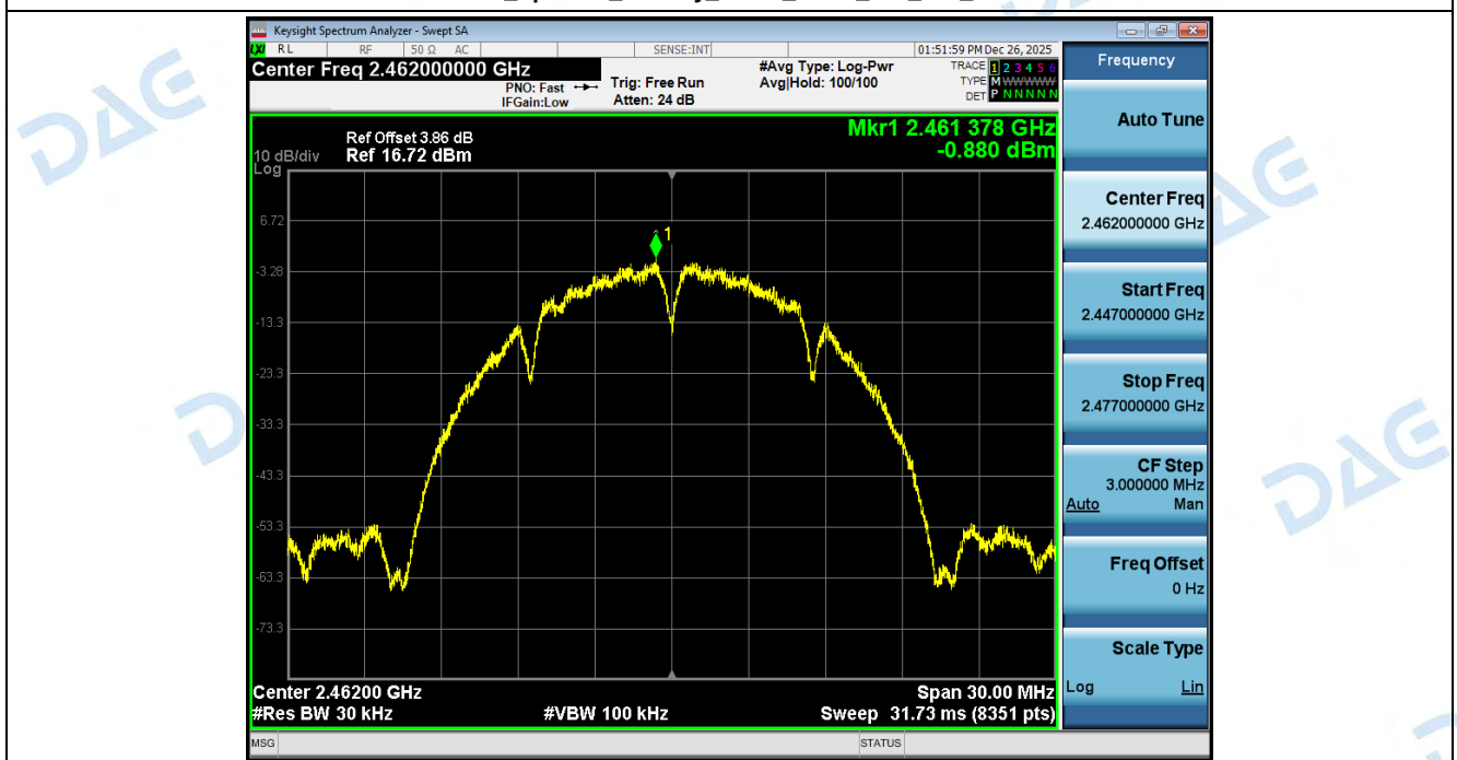
Power Spectral Density_NVNT_ANT1_802_11b_2462
