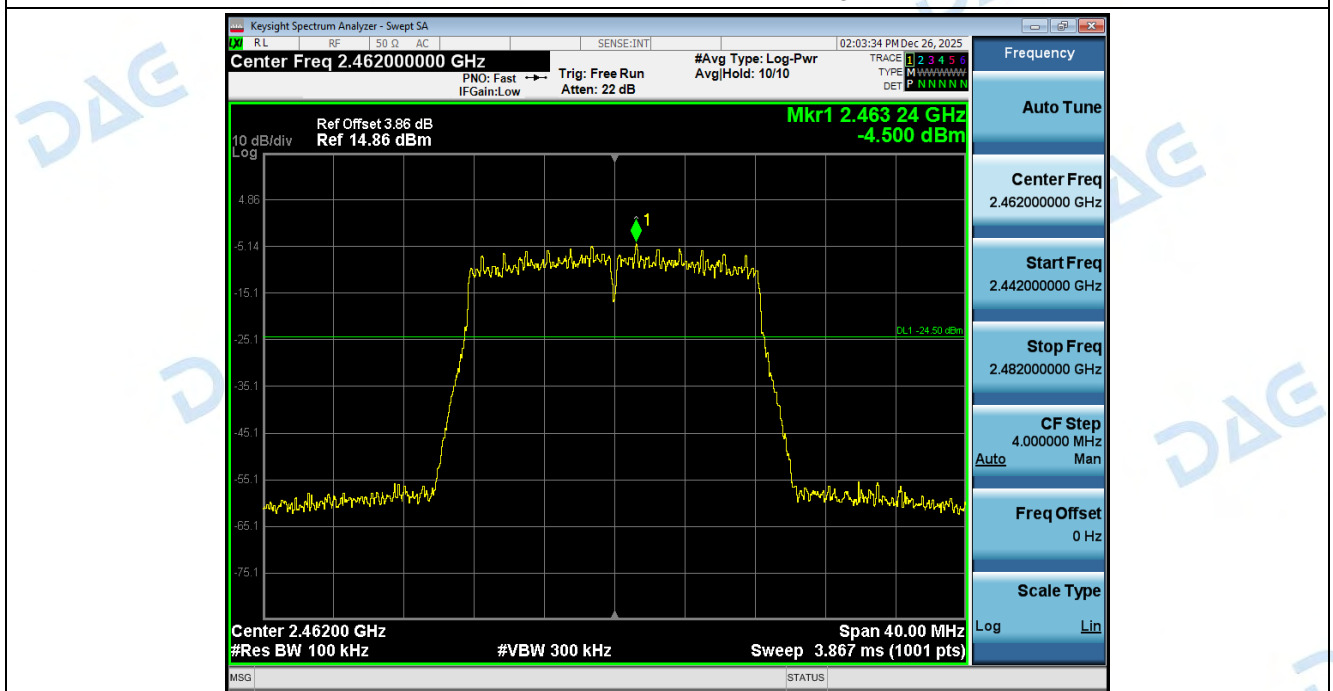
2 Bandedge_NVNT_ANT1_802_11g_2462
