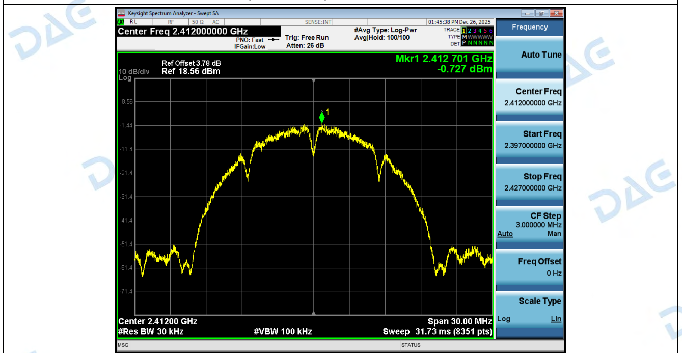
Power Spectral Density_NVNT_ANT1_802_11b_2412
