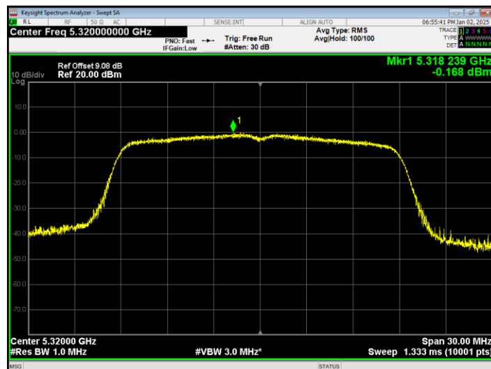
PSD NVNT ax20 5320MHz Ant2
