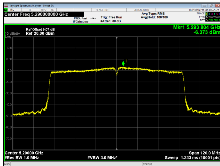
PSD NVNT ax80 5290MHz Ant2
