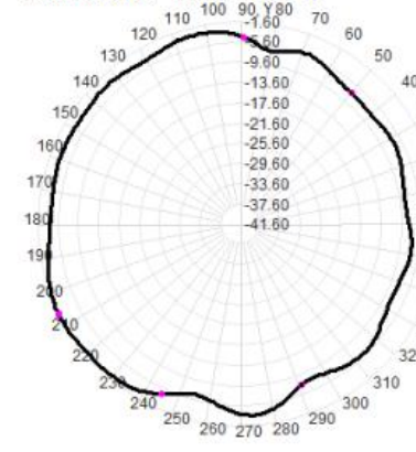
Total(H-XY), Max=-1.60dBi, CirD=7.21
