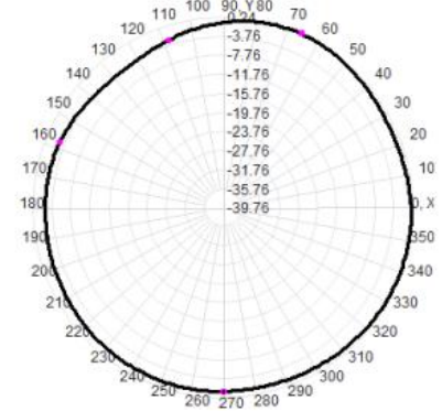
Total(H-XY), Max= 0.24dBi, CirD=4.39
