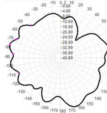
5850.0MHz H+V, Eff: 28.4%
