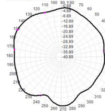
Total(H-XY), Max=-0.89dBi, CirD=7.93
