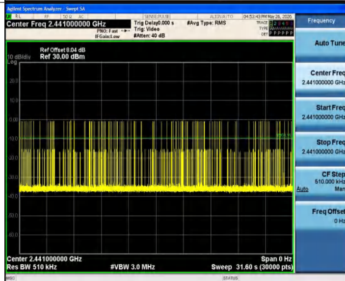
3DH5 Ant2 Hop
