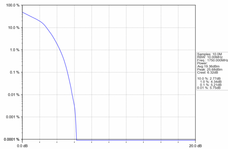
Band4_10MHz_16QAM_HCH_1750MHz_RB_50_0_NTNV
