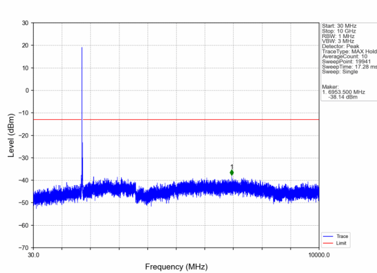
Band4_15MHz_16QAM_MCH_1732.5MHz_RB_1_0_NTNV
