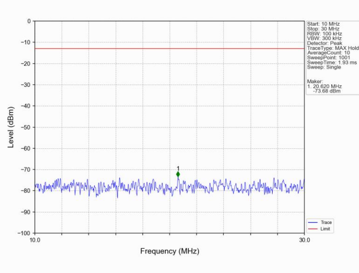
Band4_15MHz_16QAM_MCH_1732.5MHz_RB_1_0_NTNV
