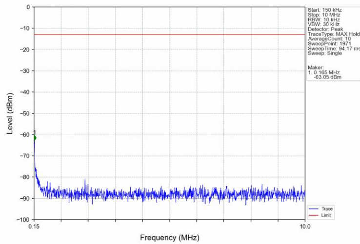
Band5_1.4MHz_QPSK_MCH_836.5MHz_RB_1_0_NTNV
