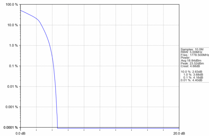
Band66 3MHz 16QAM HCH 1778.5MHz RB 15 0 NTV
