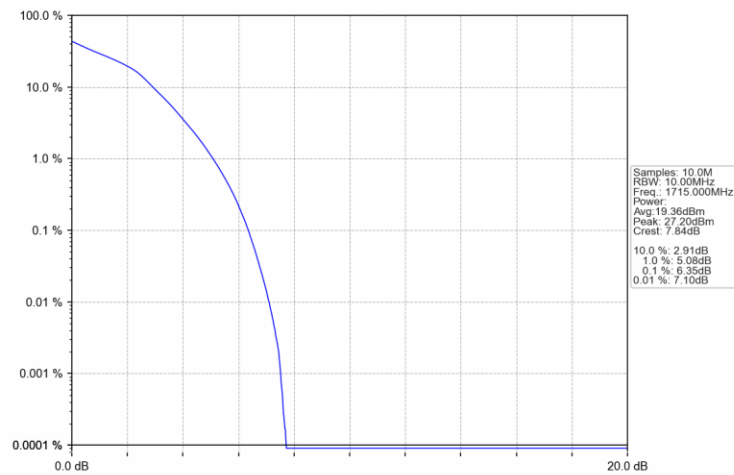
Band66 10MHz 16QAM LCH 1715MHz RB 50 0 NTV
