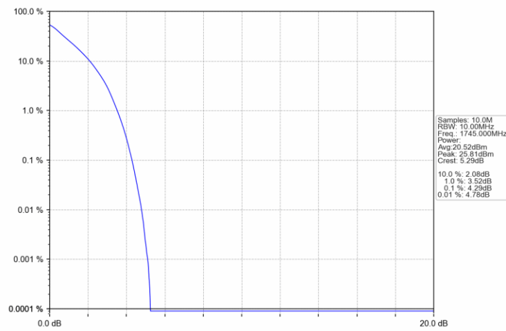
Band66_10MHz_QPSK_MCH_1745MHz_RB_50_0_NTNV
