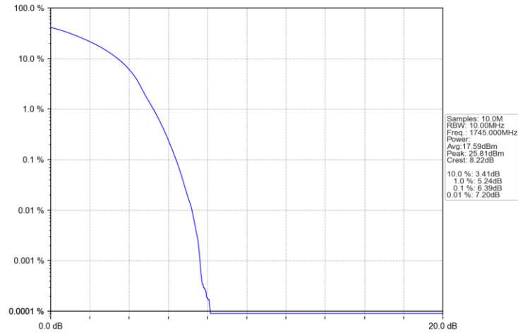
Band66 20MHz 16QAM MCH 1745MHz RB 100 0 NTNV
