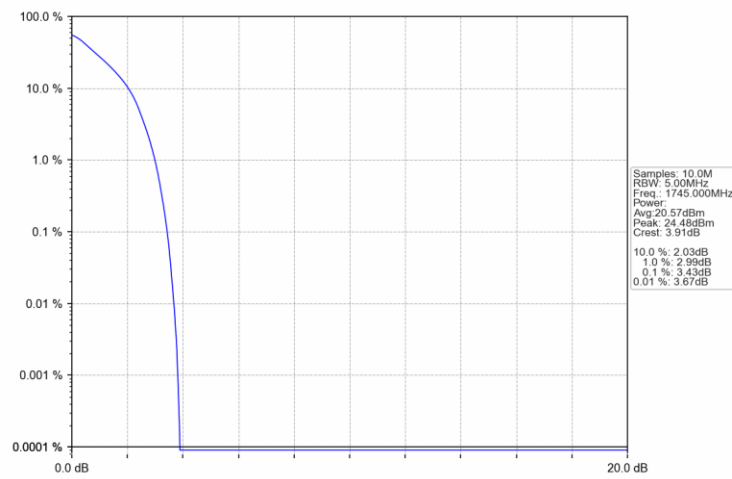
Band66_3MHz_QPSK_MCH_1745MHz_RB_15_0_NTNV
