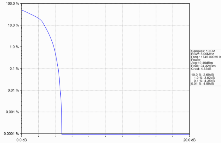
Band66 3MHz 16QAM MCH 1745MHz RB 15 0 NTV
