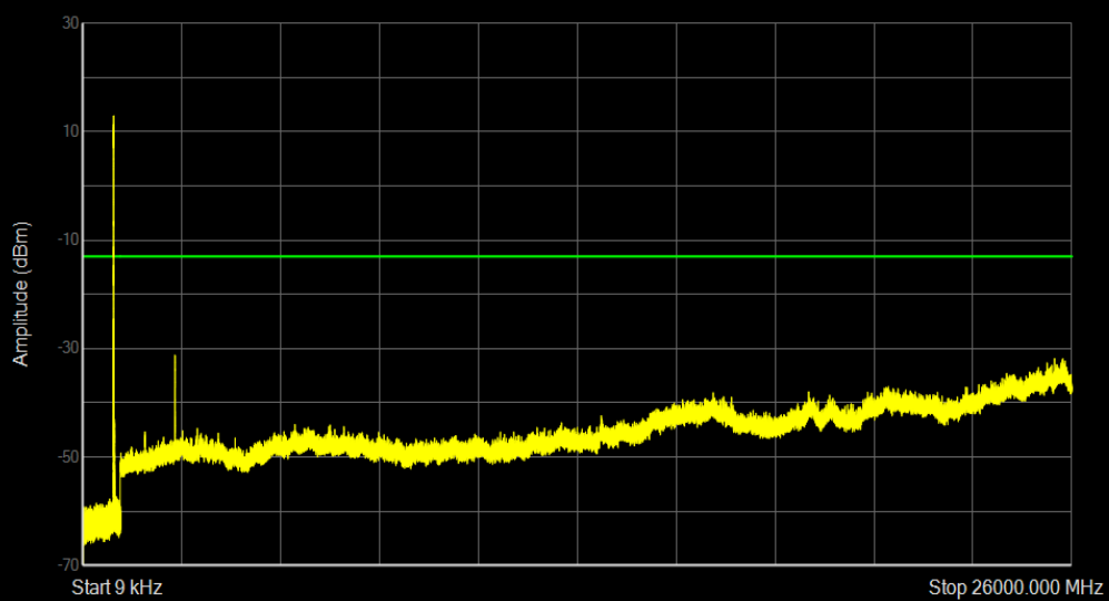
Band5 QAM16 BW=10MHz Channel=20450 RB Size=25 Position=#0
