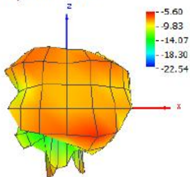
Theta = 90, Phi = 270
