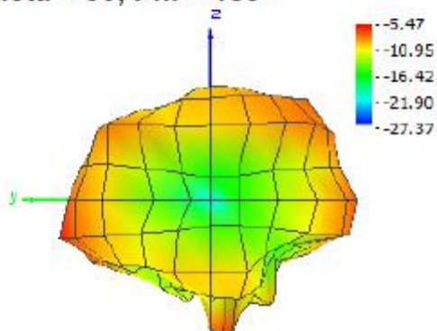
Theta = 90, Phi = 180
