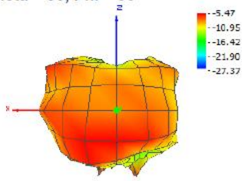
Theta = 90, Phi = 90
