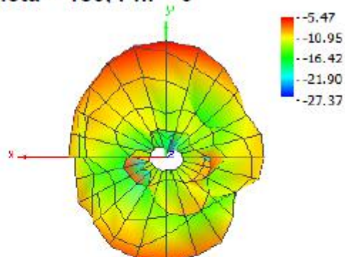
Theta = 180, Phi = 0
