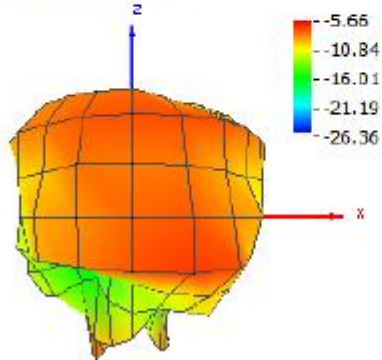
Theta = 90, Phi = 270
