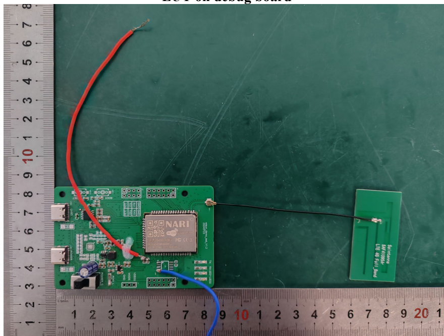
EUT on debug board
