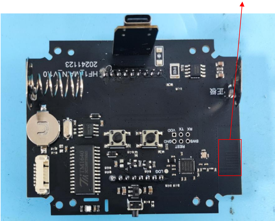
BT antenna
