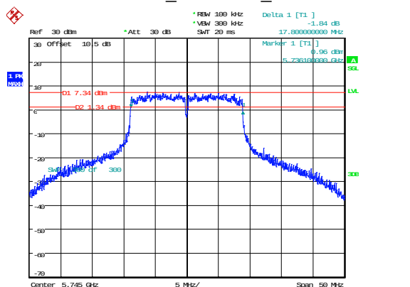
802.11n20_5745MHz_Chain 0
