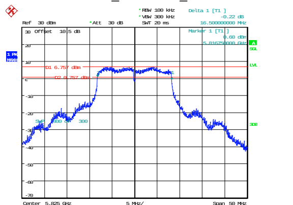
802.11a_5825MHz_Chain 0
