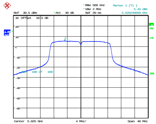
802.11n20_5825MHz_Chain 1
