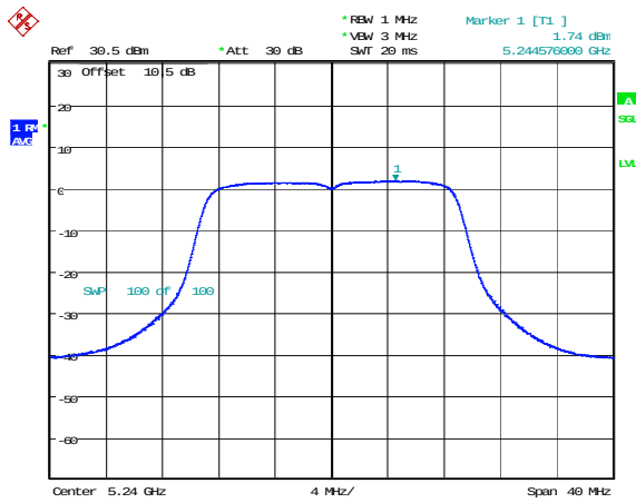
802.11n20_5240MHz_Chain 0
