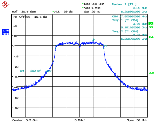
802.11n20_5200MHz_Chain 0
