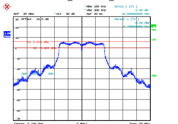
802.11a_5745MHz_Chain 0
