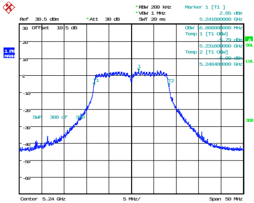
802.11a_5240MHz_Chain 0
