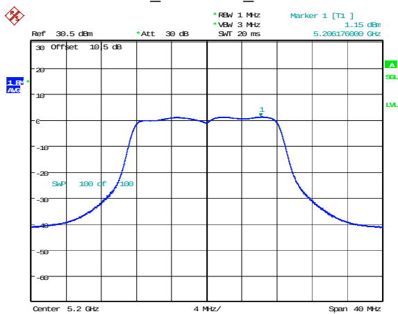
802.11a_5200MHz_Chain 1
