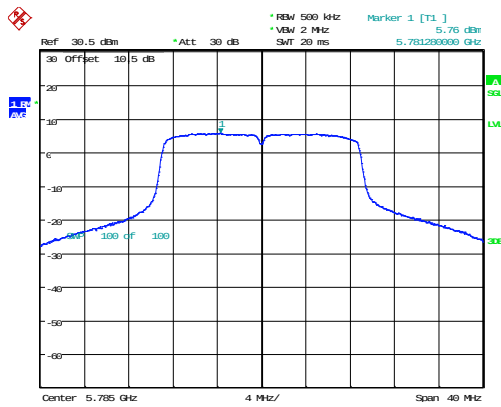
802.11n20_5785MHz_Chain 1
