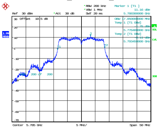
802.11a_5785MHz_Chain 0
