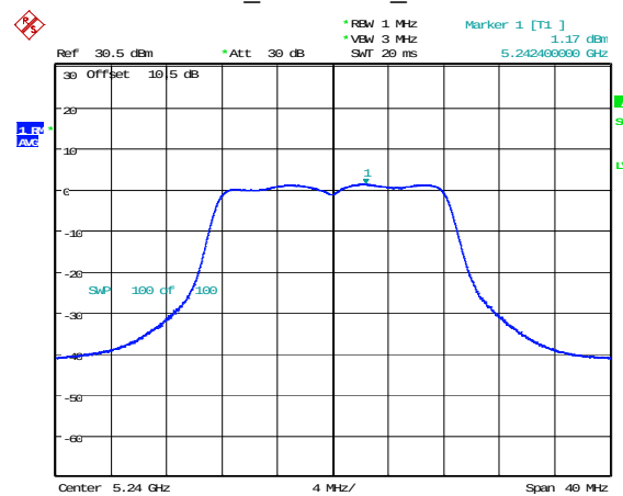
802.11a_5240MHz_Chain 1
