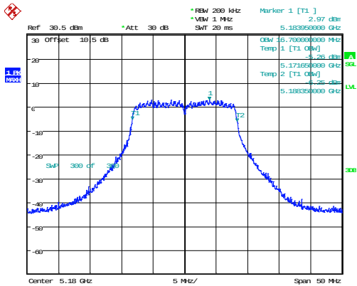
802.11a_5180MHz_Chain 0
