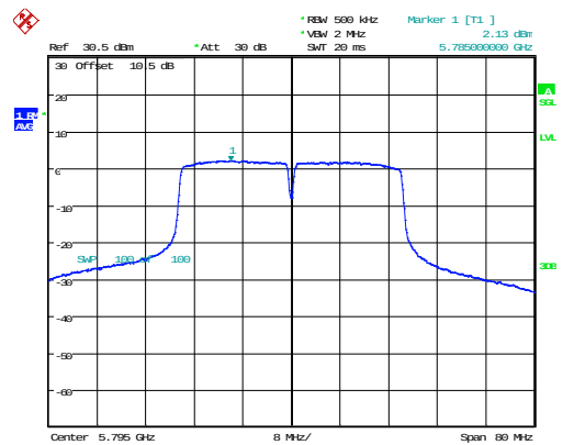
802.11n40_5795MHz_Chain 0
