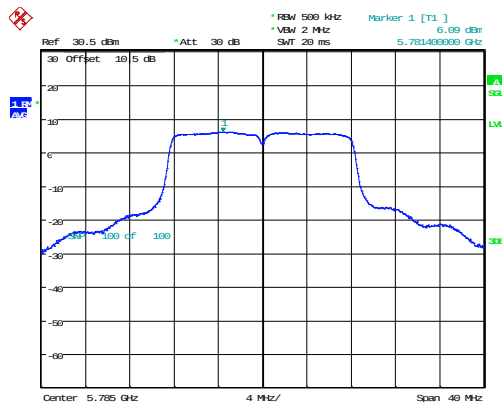
802.11a_5785MHz_Chain 1
