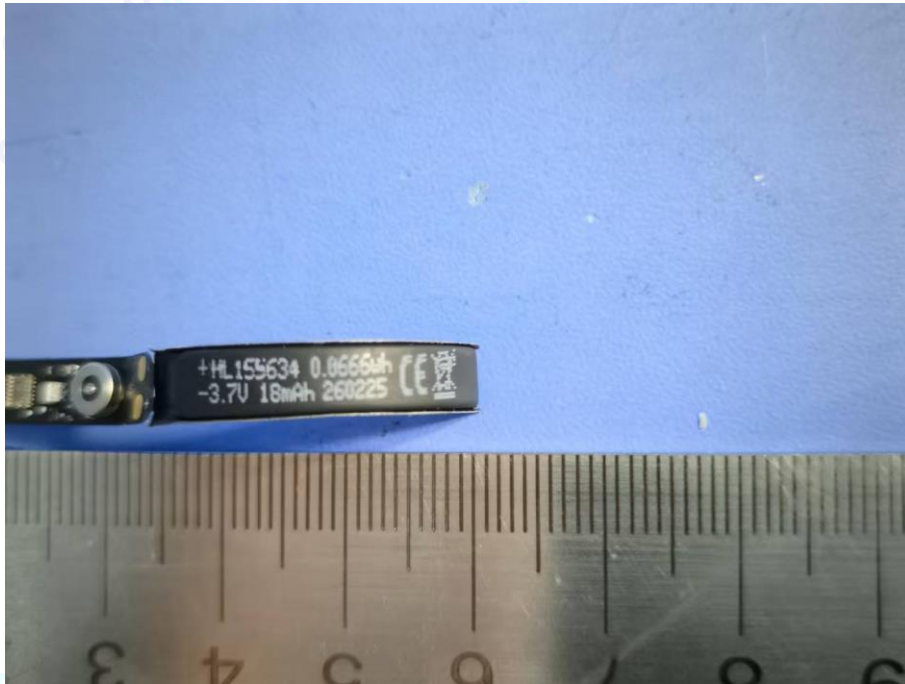
Photo 14 Battery Appearance(SF-SRA-A)
