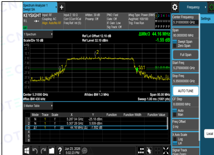
11AX40SISO-Ant1-5310
