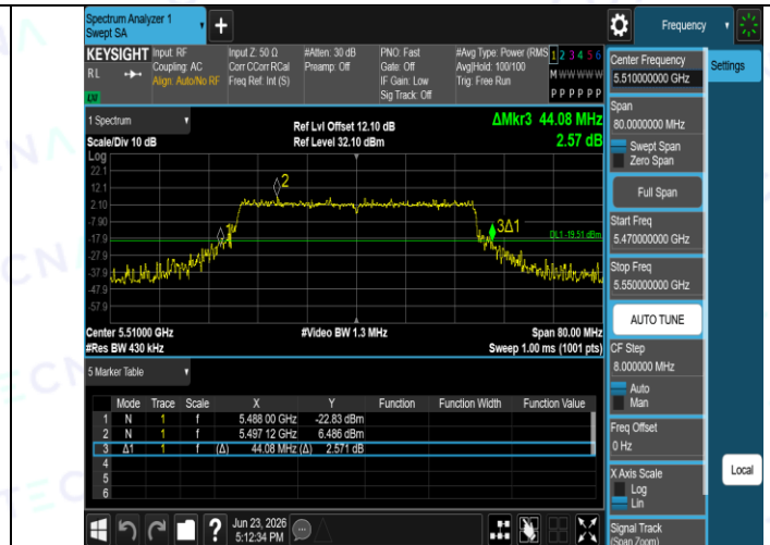
11AX40SISO-Ant1-5510
