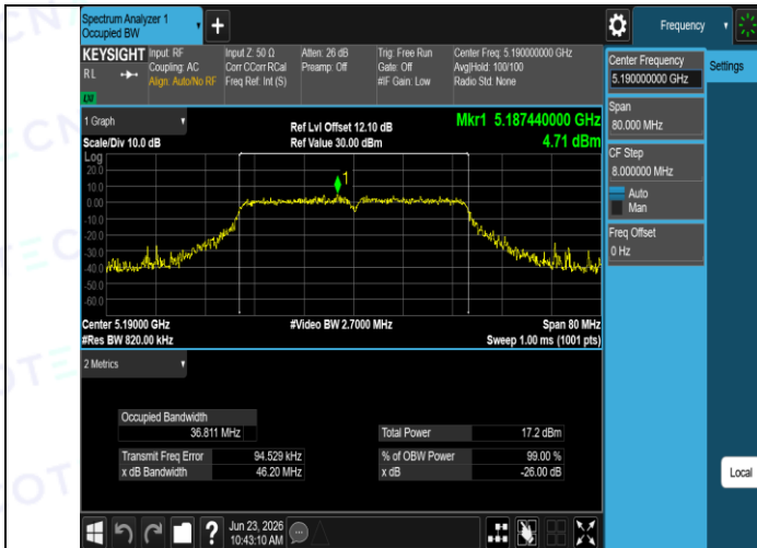
11N40SISO-Ant1-5190
