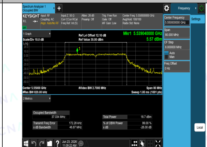
11N40SISO-Ant1-5550
