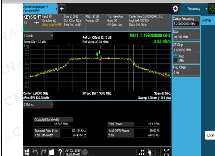
11AC20SISO-Ant1-5200
