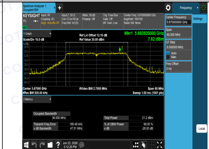
11AC40SISO-Ant1-5670
