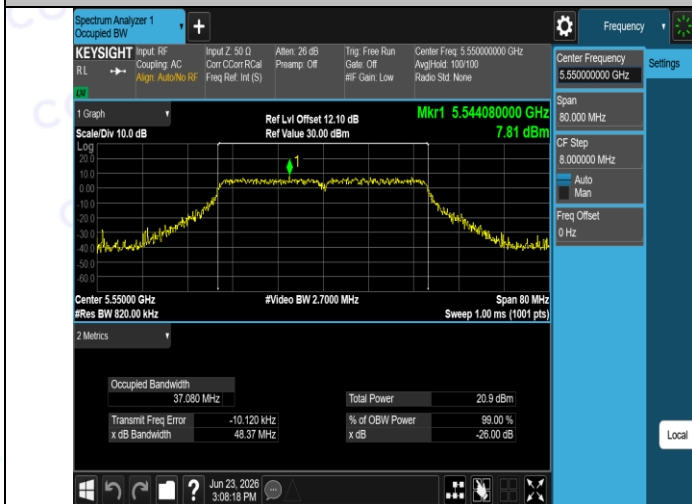
11AC40SISO-Ant1-5550
