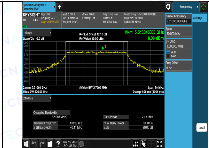
11AC40SISO-Ant1-5510
