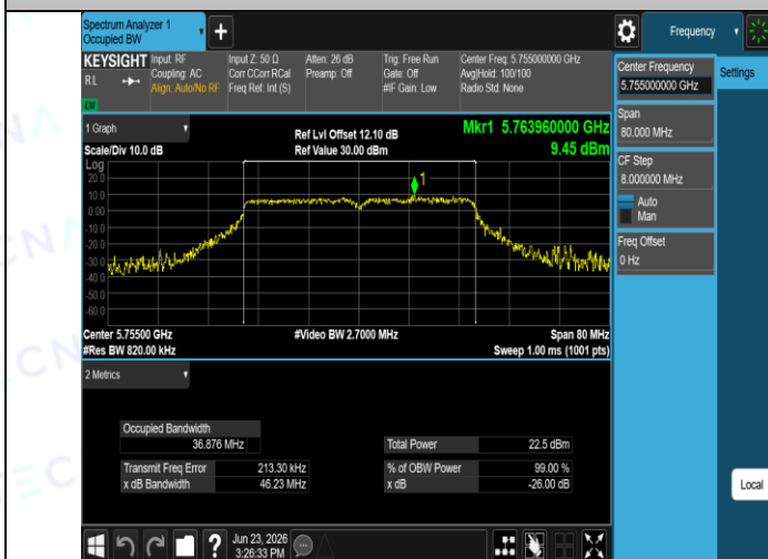
11AC40SISO-Ant1-5755
