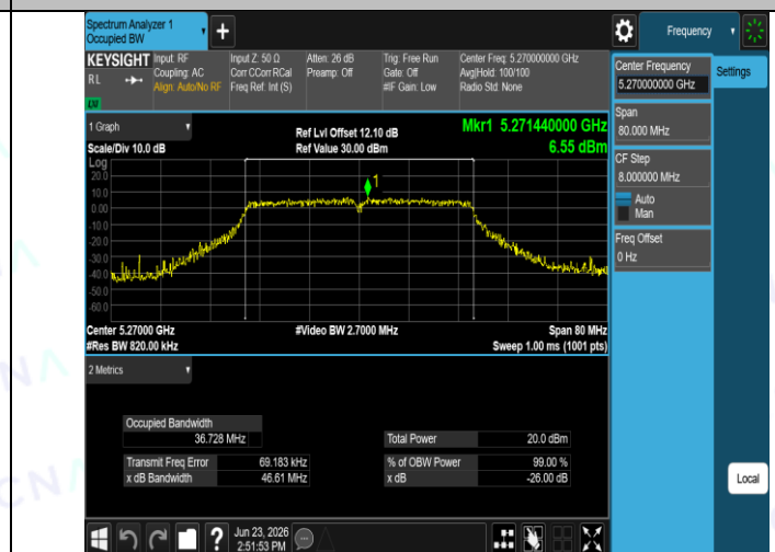
11AC40SISO-Ant1-5270
