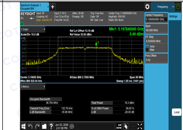
11AC40SISO-Ant1-5190
