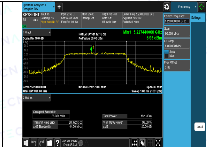
11N40SISO-Ant1-5230
