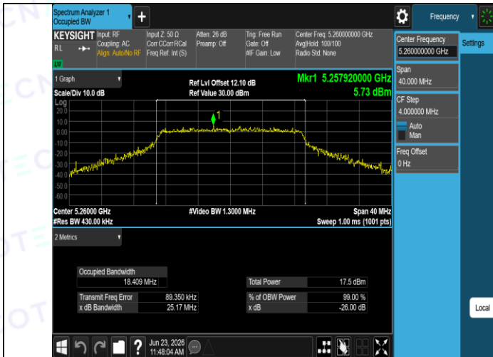
11AC20SISO-Ant1-5260
