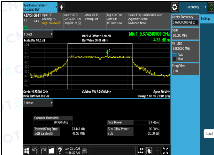
11N40SISO-Ant1-5670
