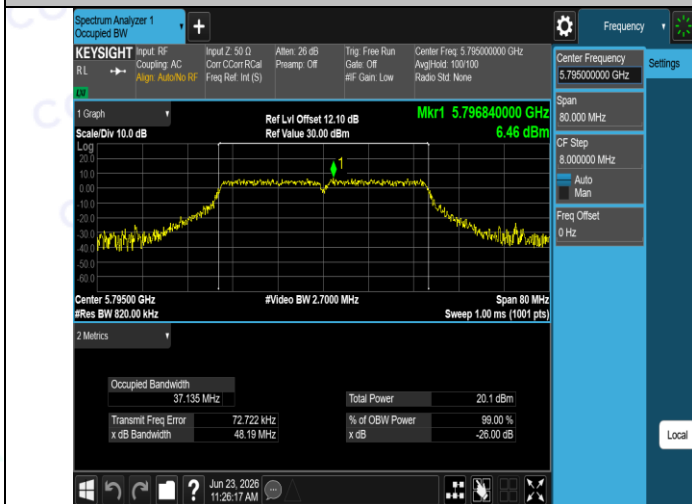
11N40SISO-Ant1-5795
