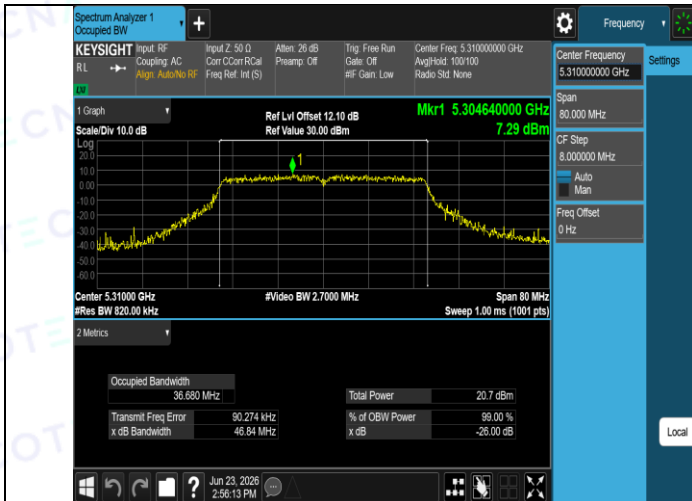
11AC40SISO-Ant1-5310
