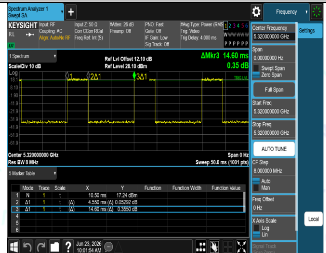
NTNV-11N20SISO-Ant1-5320
