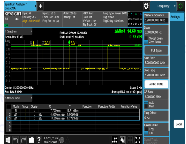
NTNV-11N20SISO-Ant1-5200
