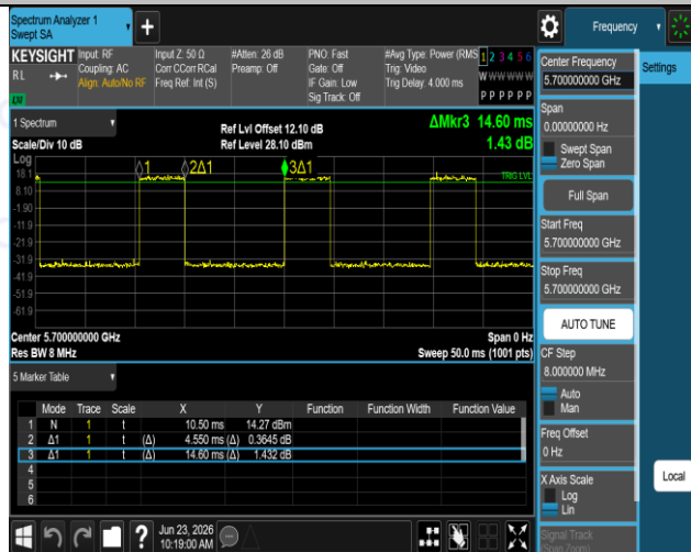
NTNV-11N20SISO-Ant1-5700
