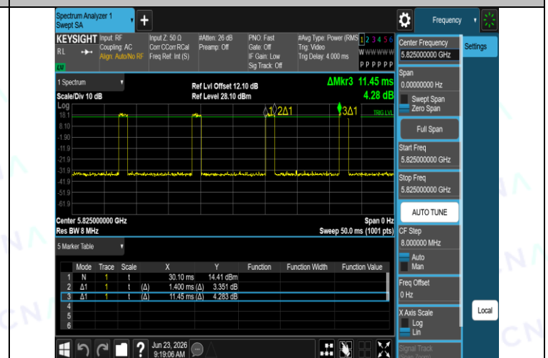
NTNV-11A-Ant1-5825
