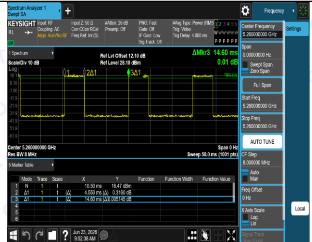
NTNV-11N20SISO-Ant1-5260
