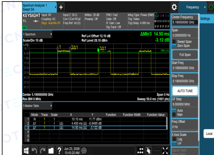
NTNV-11N40SISO-Ant1-5190
