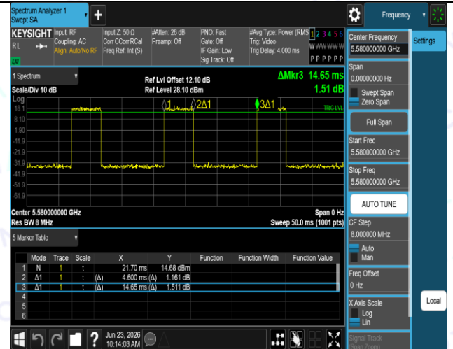
NTNV-11N20SISO-Ant1-5580
