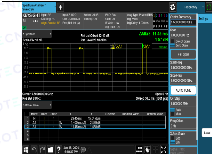
NTNV-11A-Ant1-5500
