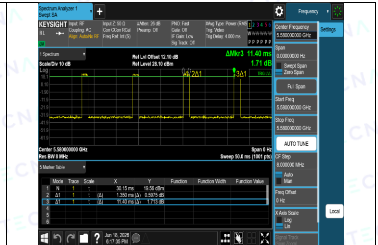
NTNV-11A-Ant1-5580
