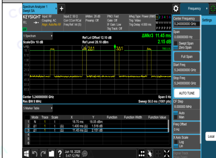
NTNV-11A-Ant1-5240
