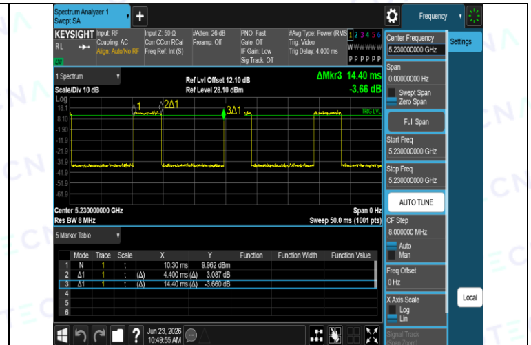
NTNV-11N40SISO-Ant1-5230
