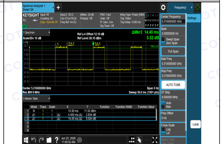
NTNV-11N40SISO-Ant1-5310
