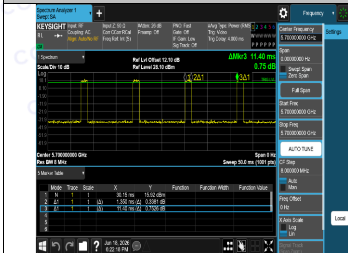
NTNV-11A-Ant1-5700
