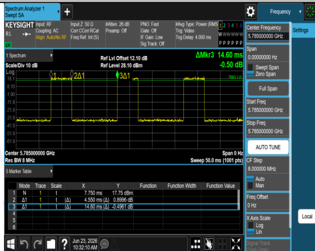
NTNV-11N20SISO-Ant1-5785
