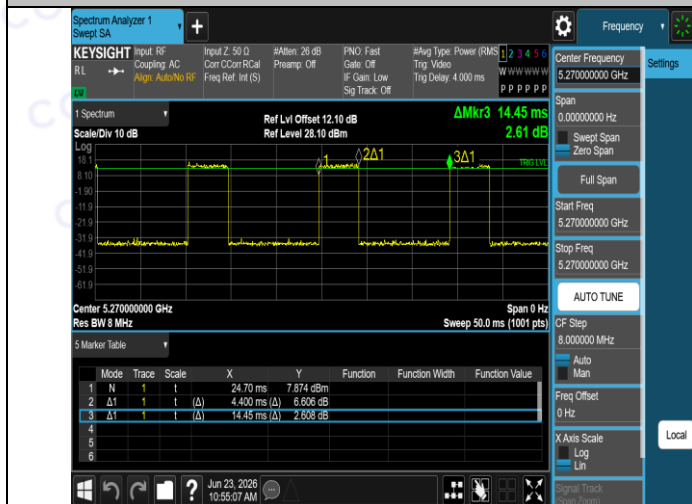
NTNV-11N40SISO-Ant1-5270
