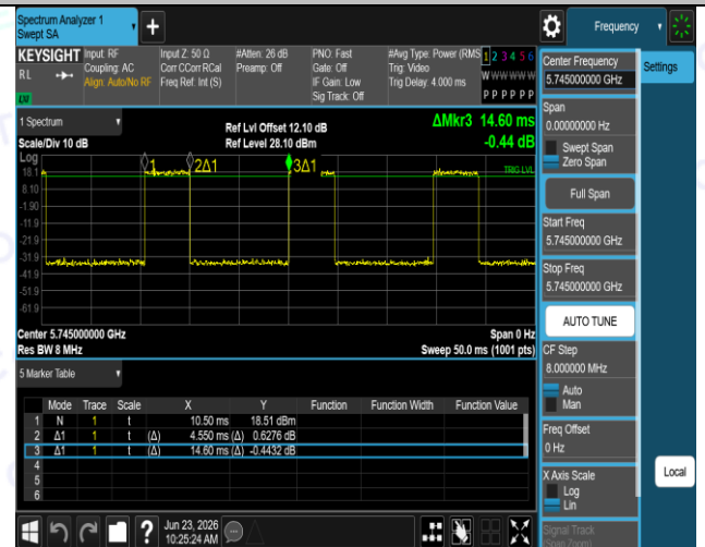
NTNV-11N20SISO-Ant1-5745
