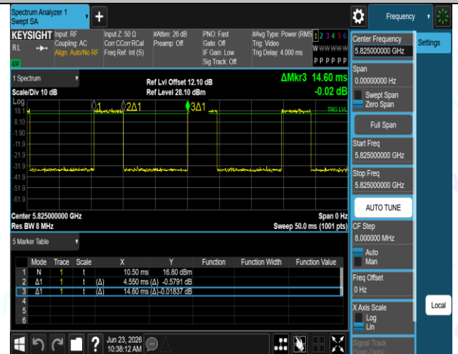
NTNV-11N20SISO-Ant1-5825
