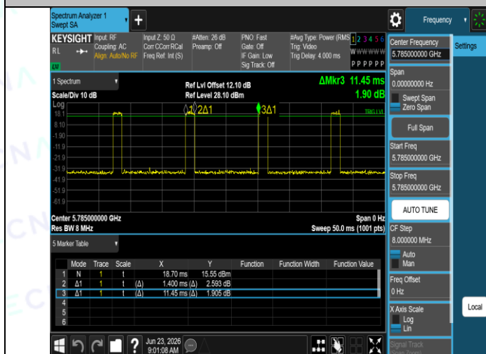
NTNV-11A-Ant1-5785
