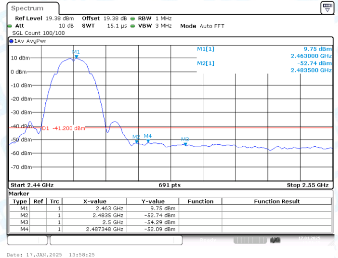
11B-Ant1-2462-PASS
