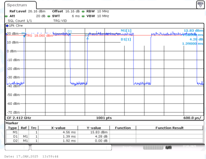
NTNV-11G-Ant1-2412
