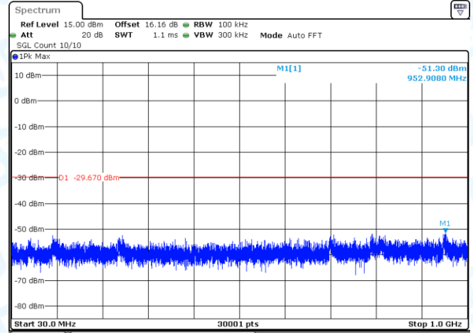
11AX20SISO-Ant1-2412-30~1000-PASS
