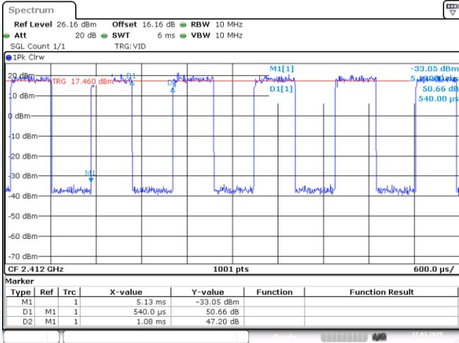
NTNV-11N20SISO-Ant1-2412
