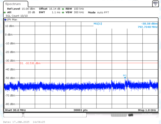
11AX20SISO-Ant1-2462-30~1000-PASS
