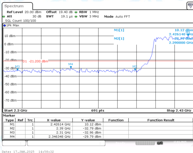
11AX40SISO-Ant1-2422-PASS
