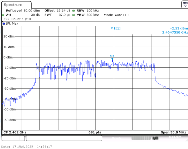
11AX20SISO-Ant1-2462-0~Reference-PASS
