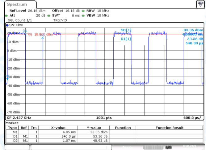
NTNV-11N20SISO-Ant1-2437
