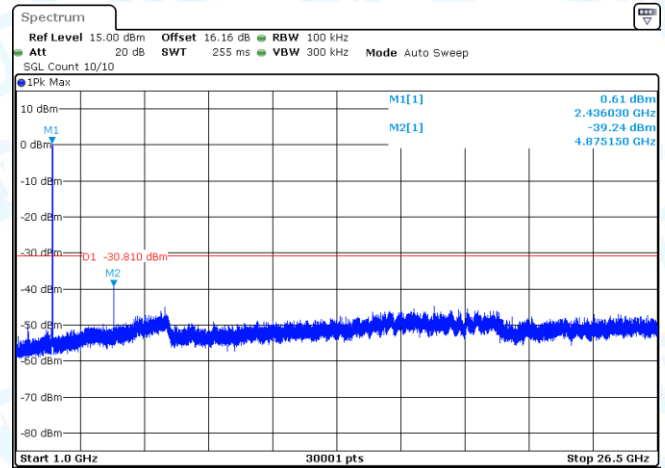
11AX20SISO-Ant1-2437-0~Reference-PASS
