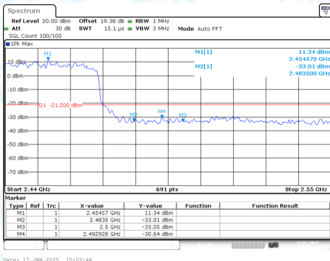
11AX40SISO-Ant1-2452-PASS
