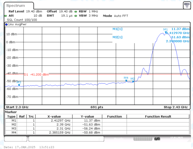
11B-Ant1-2412-PASS
