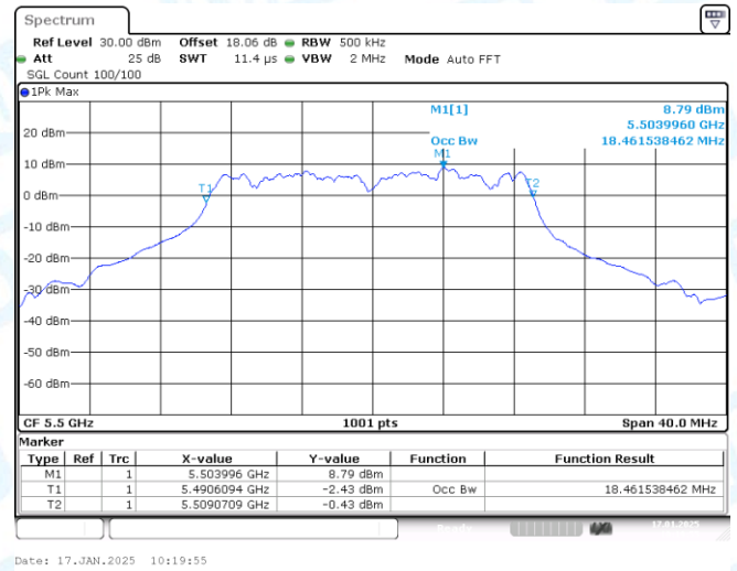
11AC20SISO-Ant1-5500
