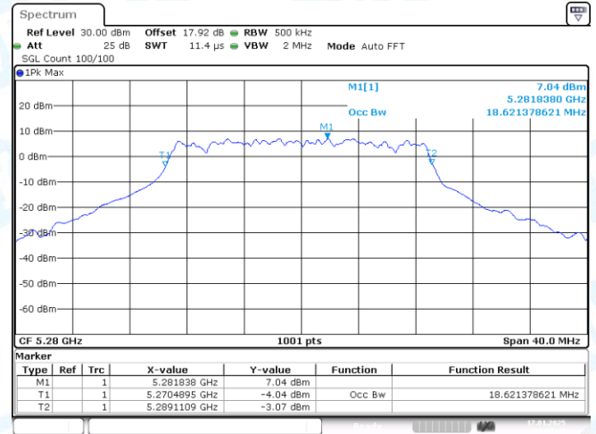
11AC20SISO-Ant1-5280
