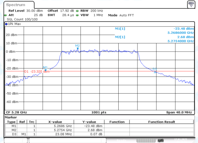
11N20SISO-Ant1-5280
