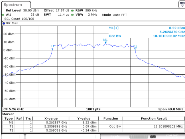
11AC20SISO-Ant1-5260
