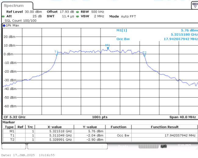
11AC20SISO-Ant1-5320
