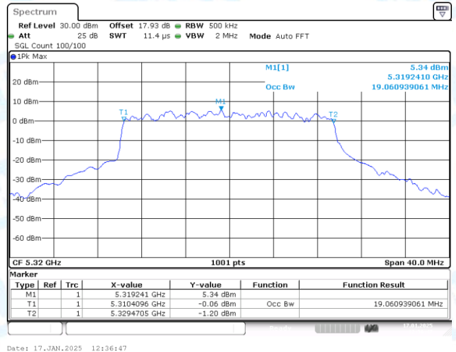
11AX20SISO-Ant1-5320
