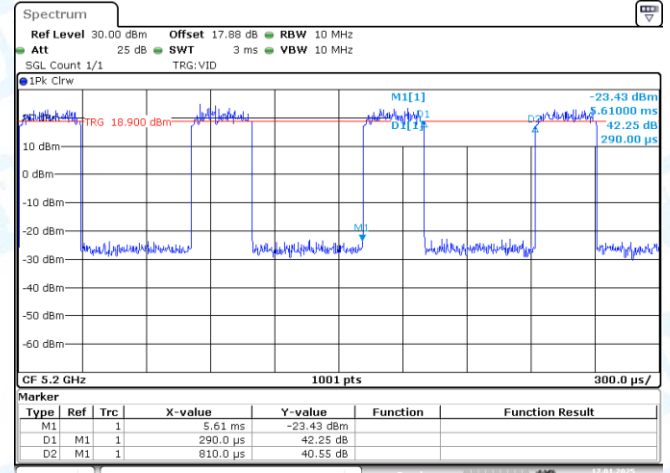
NTNV-11AX20SISO-Ant1-5200
