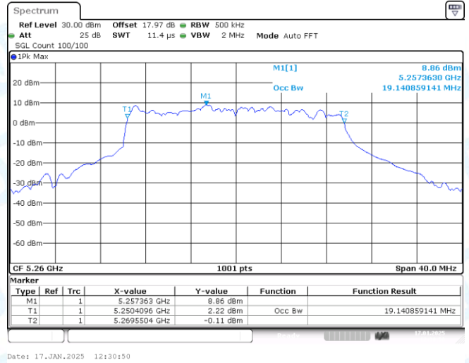
11AX20SISO-Ant1-5260
