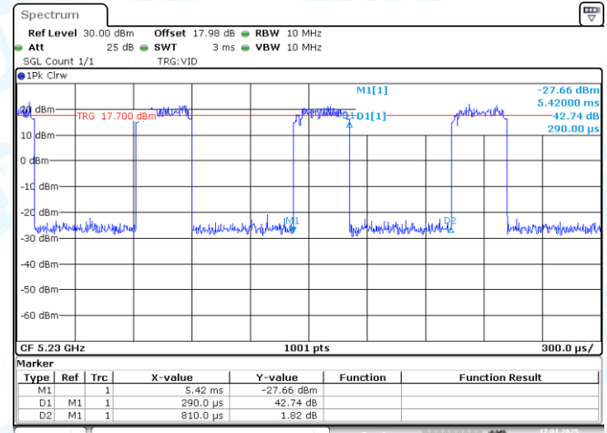
NTNV-11AX40SISO-Ant1-5230
