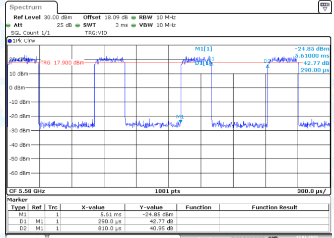
NTNV-11AX20SISO-Ant1-5580
