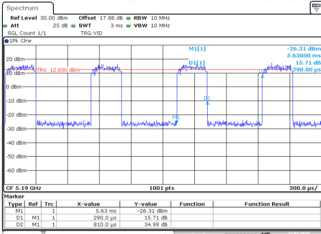
NTNV-11AX40SISO-Ant1-5190
