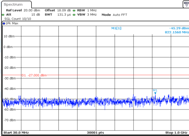
11A-Ant1-5500-30~1000-PASS
