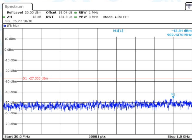
11N40SISO-Ant1-5310-30~1000-PASS
