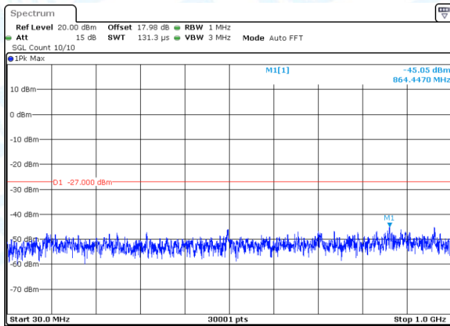
11AX20SISO-Ant1-5200-30~1000-PASS
