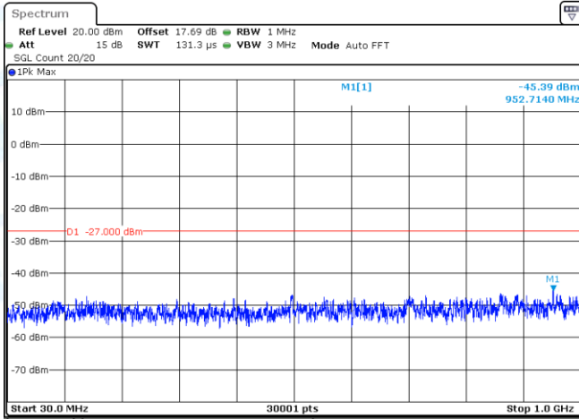
11N20SISO-Ant1-5745-30~1000-PASS
