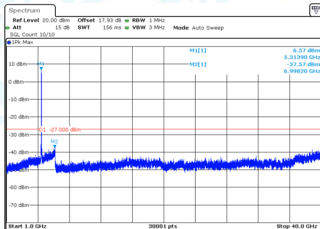
11N40SISO-Ant1-5310-1000~40000-PASS
