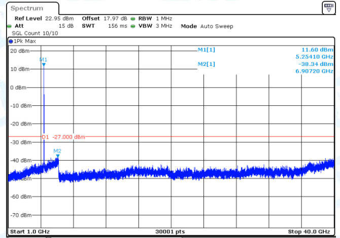
11AC20SISO-Ant1-5260-1000~40000-PASS
