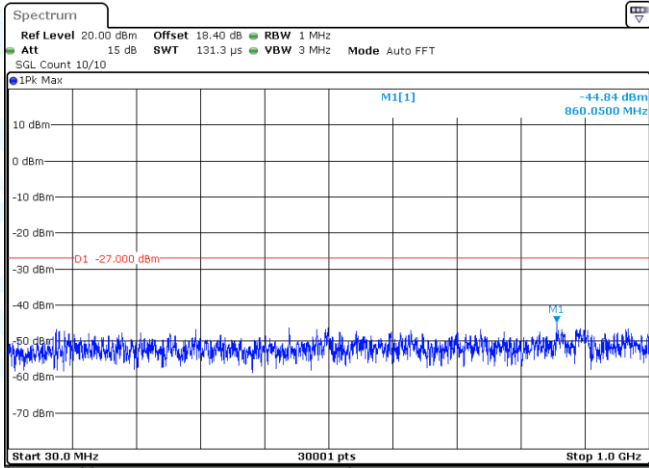
11N20SISO-Ant1-5580-30~1000-PASS
