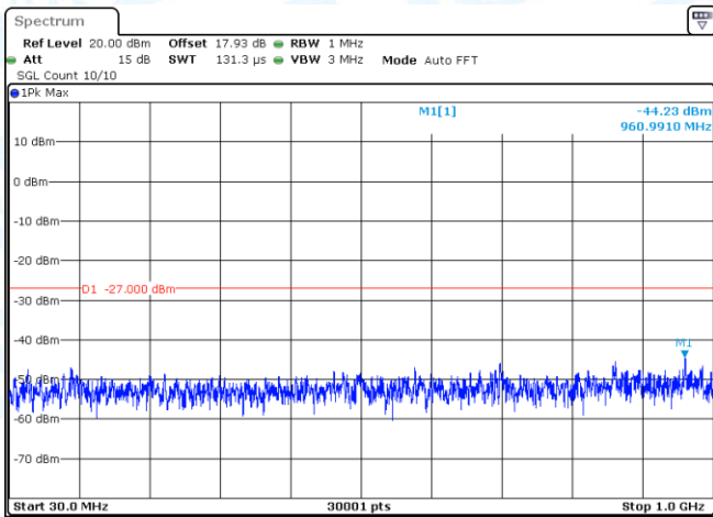
11N20SISO-Ant1-5280-30~1000-PASS
