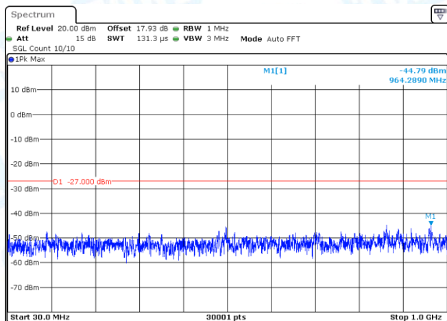
11N40SISO-Ant1-5310-30~1000-PASS
