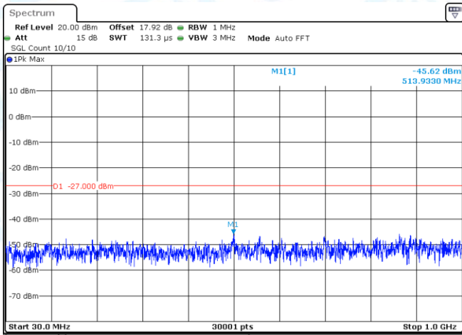
11AX20SISO-Ant1-5260-30~1000-PASS
