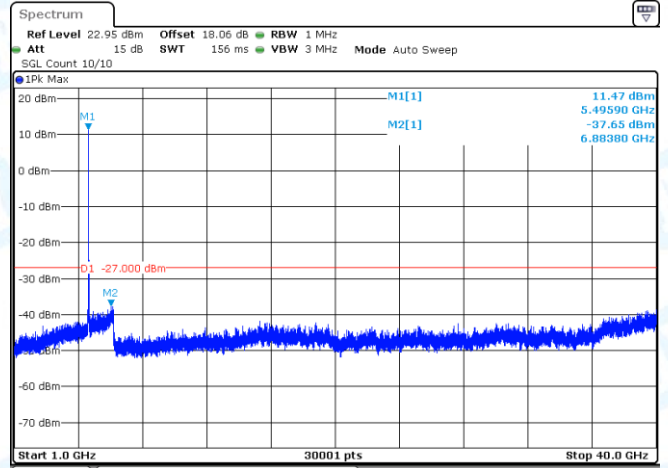
11AC20SISO-Ant1-5500-1000~40000-PASS
