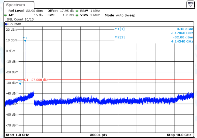
11AX20SISO-Ant1-5180-1000~40000-PASS
