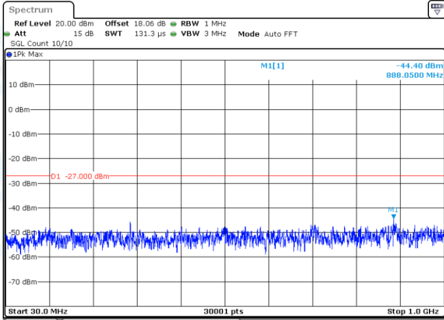
11N20SISO-Ant1-5500-30~1000-PASS
