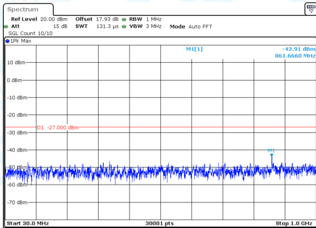
11A-Ant1-5280-30~1000-PASS
