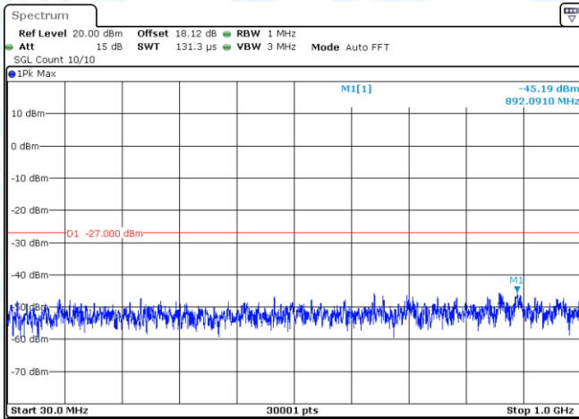
11AC40SISO-Ant1-5510-30~1000-PASS
