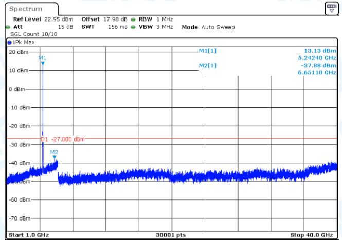
11N20SISO-Ant1-5200-1000~40000-PASS
