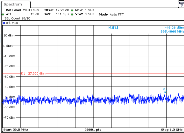
11N40SISO-Ant1-5230-30~1000-PASS
