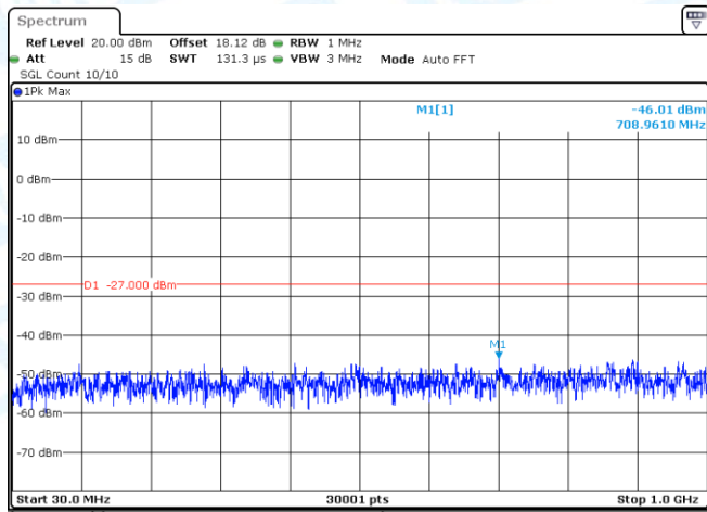
11N40SISO-Ant1-5510-30~1000-PASS
