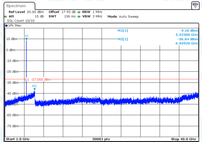
11AC20SISO-Ant1-5280-1000~40000-PASS
