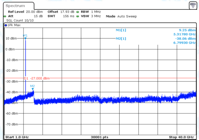
11A-Ant1-5280-1000~40000-PASS
