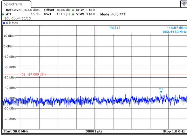
11AC20SISO-Ant1-5500-30~1000-PASS
