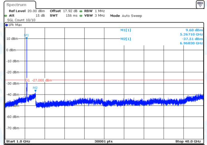
11N40SISO-Ant1-5230-1000~40000-PASS
