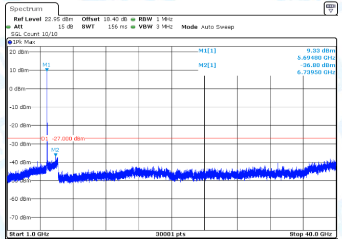
11AC20SISO-Ant1-5580-1000~40000-PASS
