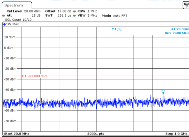
11AX20SISO-Ant1-5180-30~1000-PASS
