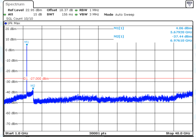
11AC40SISO-Ant1-5670-1000~40000-PASS
