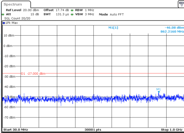
11N20SISO-Ant1-5785-30~1000-PASS
