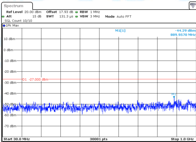
11AX20SISO-Ant1-5280-30~1000-PASS
