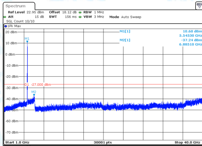
11N40SISO-Ant1-5510-1000~40000-PASS
