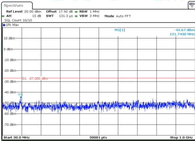
11N20SISO-Ant1-5260-30~1000-PASS
