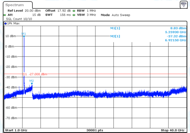
11AC40SISO-Ant1-5230-1000~40000-PASS
