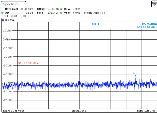
11AC20SISO-Ant1-5580-30~1000-PASS
