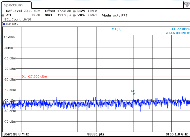
11AC40SISO-Ant1-5230-30~1000-PASS
