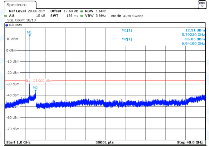
11N20SISO-Ant1-5745-1000~40000-PASS
