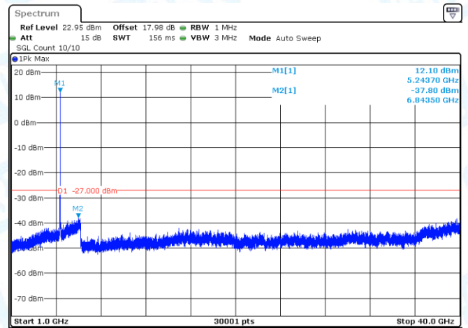
11AX20SISO-Ant1-5200-1000~40000-PASS
