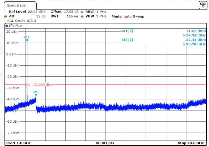
11AC20SISO-Ant1-5200-1000~40000-PASS
