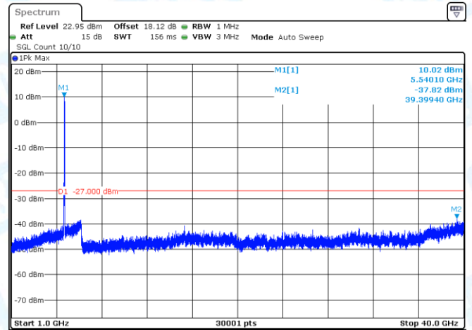
11AC40SISO-Ant1-5510-1000~40000-PASS
