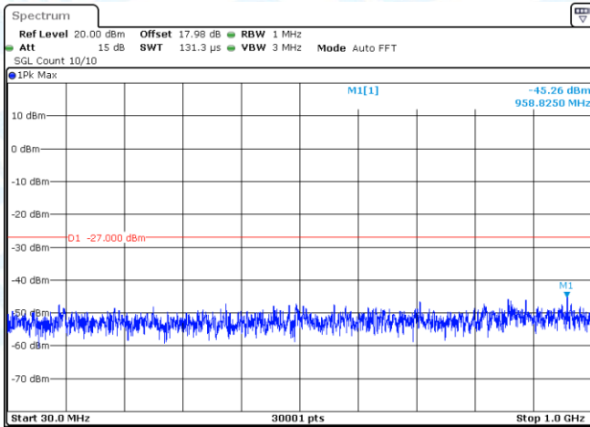
11AC20SISO-Ant1-5200-30~1000-PASS
