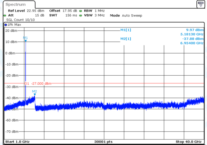
11N20SISO-Ant1-5180-1000~40000-PASS
