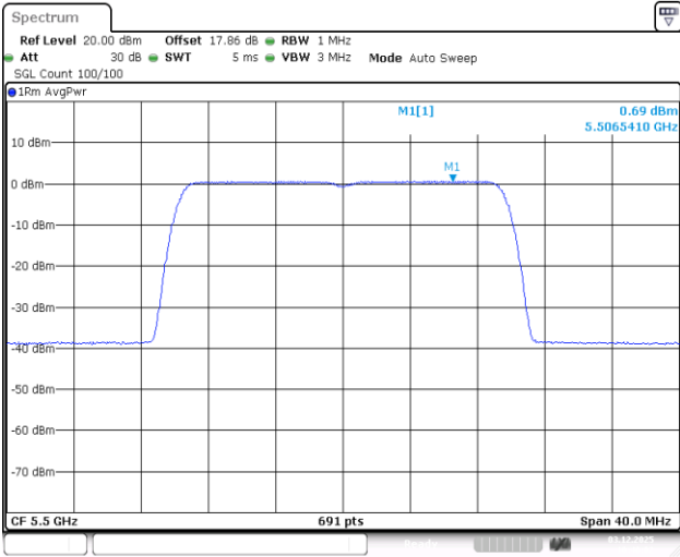
11AX20SISO-Ant1-5500-PASS
