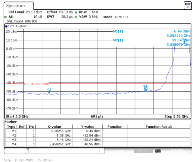
11A-Ant1-5500-PASS
