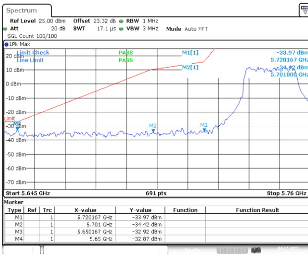
11AC40SISO-Ant1-5755-PASS
