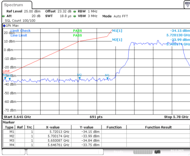
11AX40SISO-Ant1-5755-PASS
