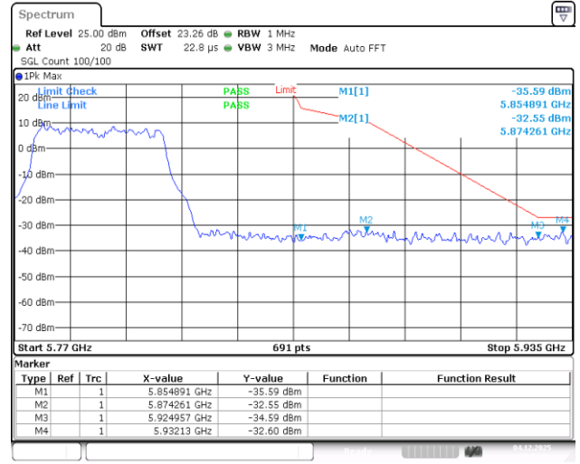
11AX40SISO-Ant1-5795-PASS
