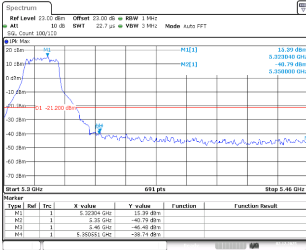
11N20SISO-Ant1-5320-PASS
