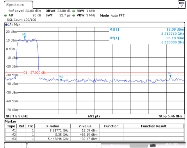
11AC20SISO-Ant1-5320-PASS
