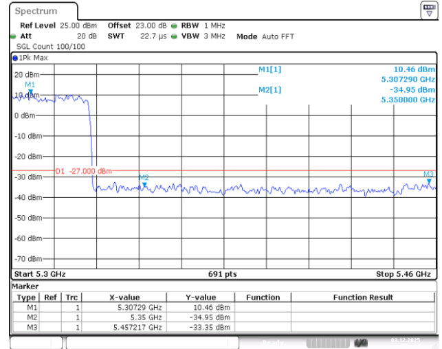
11AX40SISO-Ant1-5310-PASS
