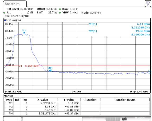
11N20SISO-Ant1-5320-PASS
