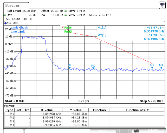
11AX20SISO-Ant1-5825-PASS
