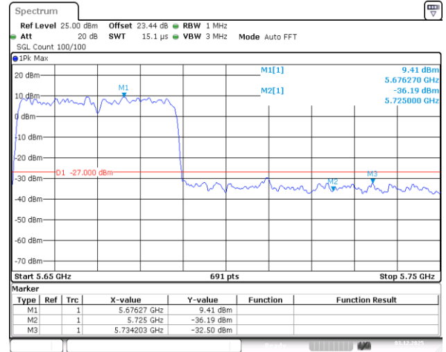
11AC40SISO-Ant1-5670-PASS
