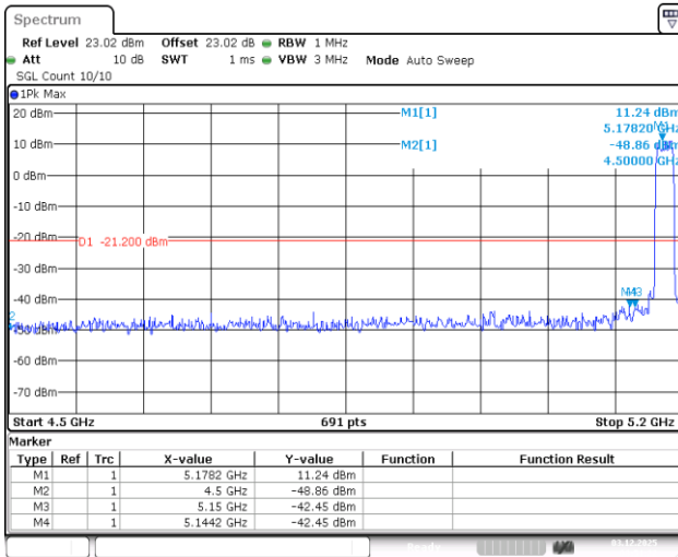
11AC20SISO-Ant1-5180-PASS
