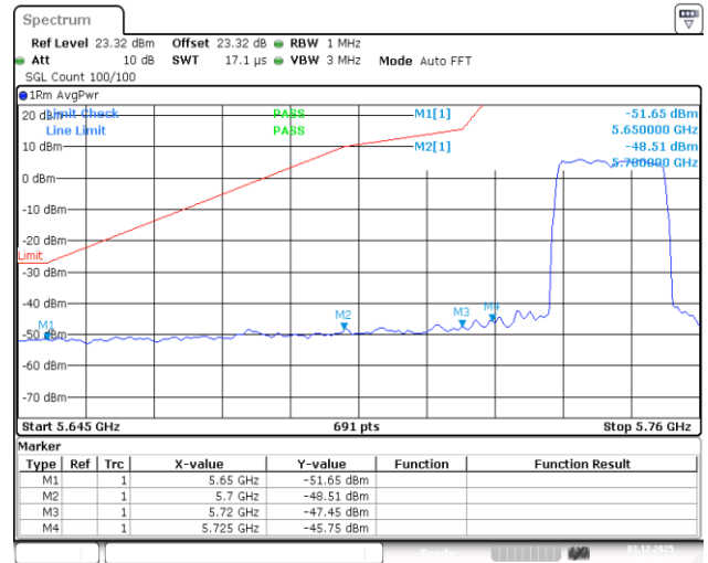
11AC20SISO-Ant1-5745-PASS
