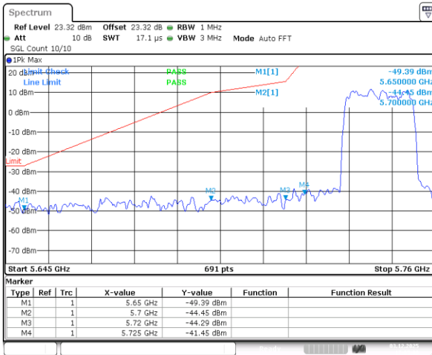
11AC20SISO-Ant1-5745-PASS
