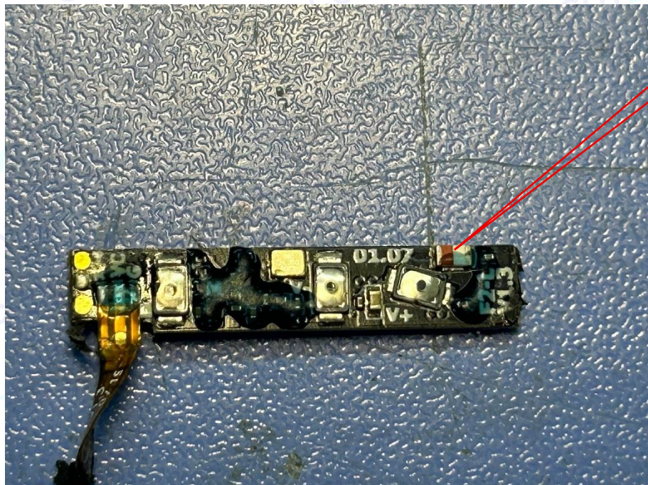
Photo 17 Appearance of PCB-L
