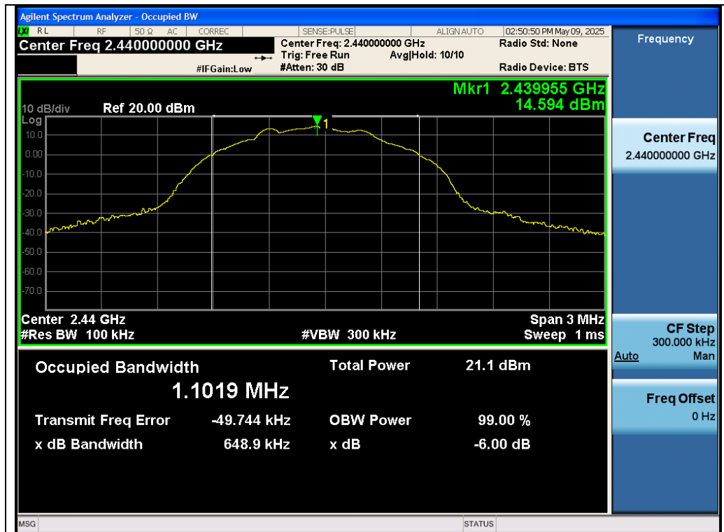
Test_Graph_LE125K_ANT1_2440_125Kbps_DTSBW
