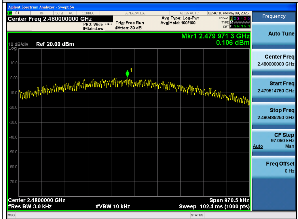
Test_Graph_LE125K_ANT1_2480_125Kbps_PSD
