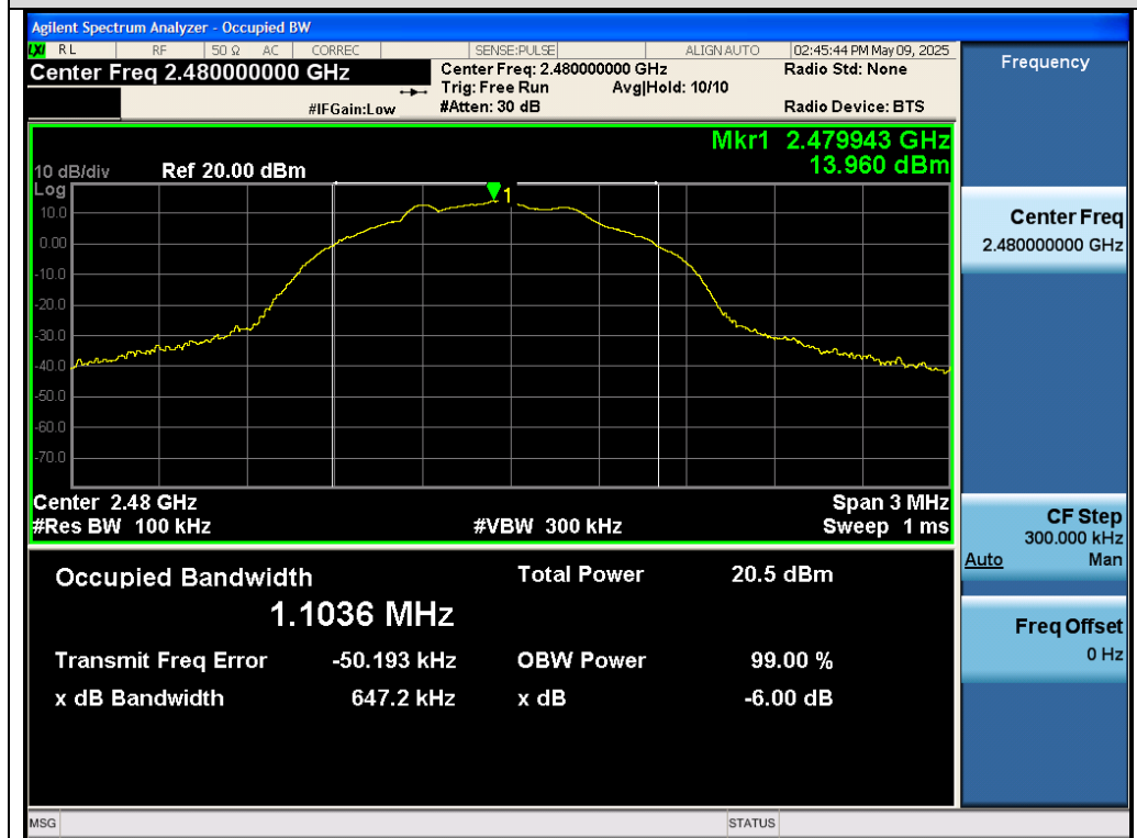
Test_Graph_LE125K_ANT1_2480_125Kbps_DTSBW
