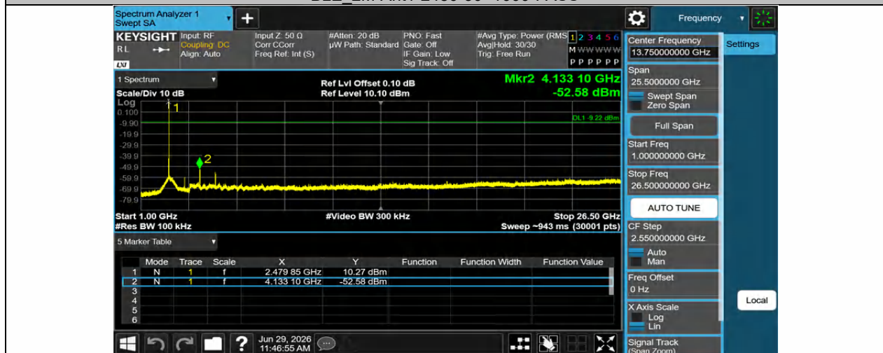
BLE_2M-Ant1-2480-1000~26500-PASS
