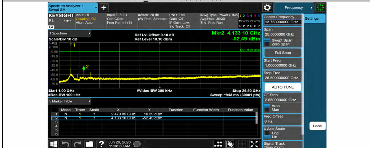
BLE_1M-Ant1-2480-1000~26500-PASS
