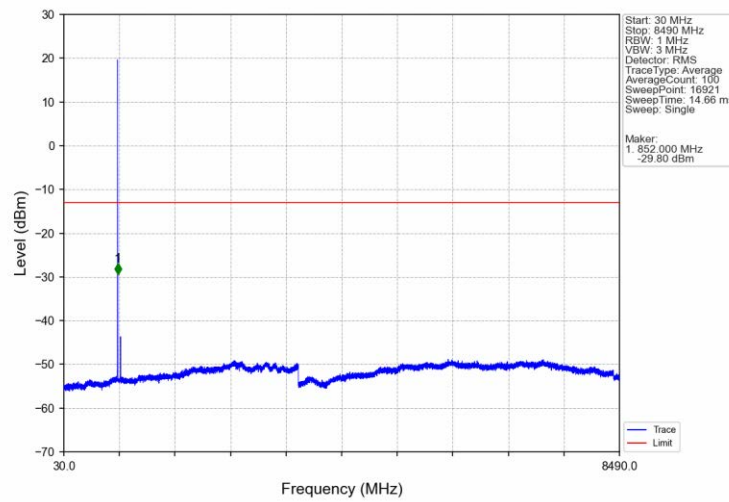
Band5_1.4MHz_16QAM_HCH_848.3MHz_RB_1_0_NTNV
