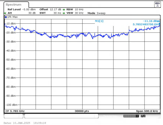
NT/NV_Antenna 0 IEEE 802.11n_Channel 157_20MHz
