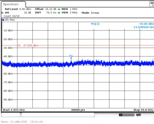
Spurious Emission:5925~25000.0 MHz IEEE 802.11a_Channel 165_20MHz_Antenna 0
