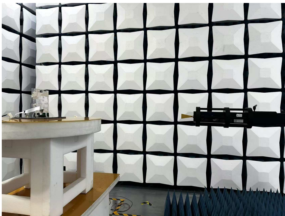
Photograph 4: Set-up photo for Radiated Spurious Emission, above 40GHz
