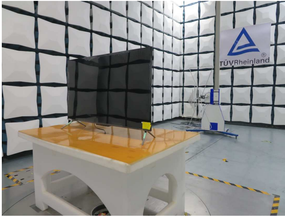
Photograph 6: Set-up photo for Radiated Spurious Emission, Below 1GHz
