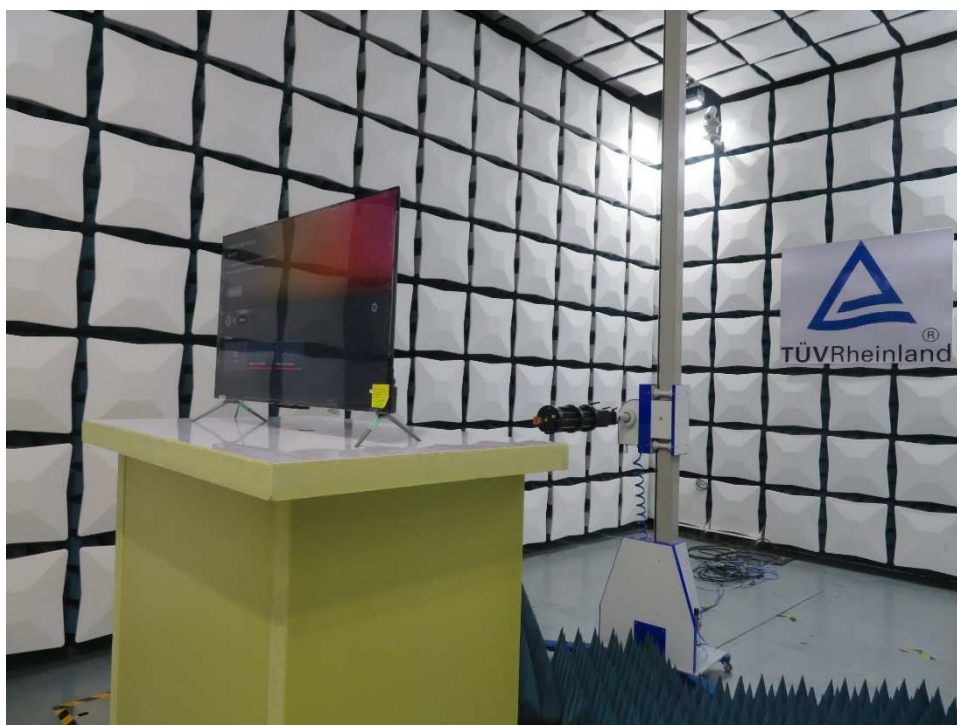
Photograph 9: Set-up photo for Radiated Spurious Emission, above 40GHz
