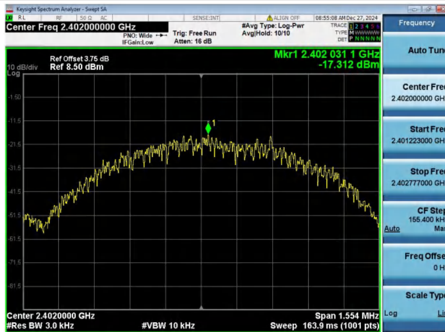
Power_Spectral_Density_NVNT_ANT1_1Mbps_2402
