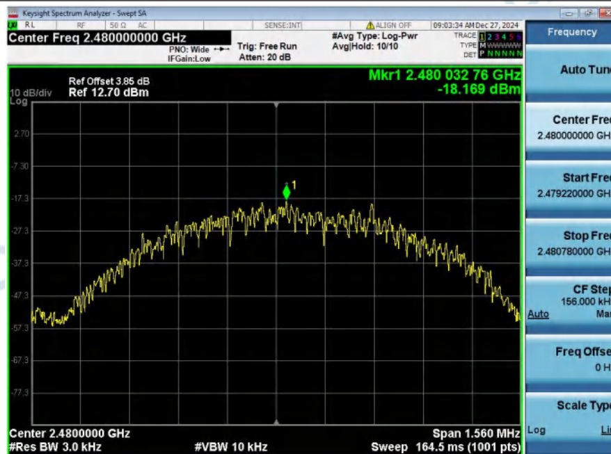
Power_Spectral_Density_NVNT_ANT1_1Mbps_2480
