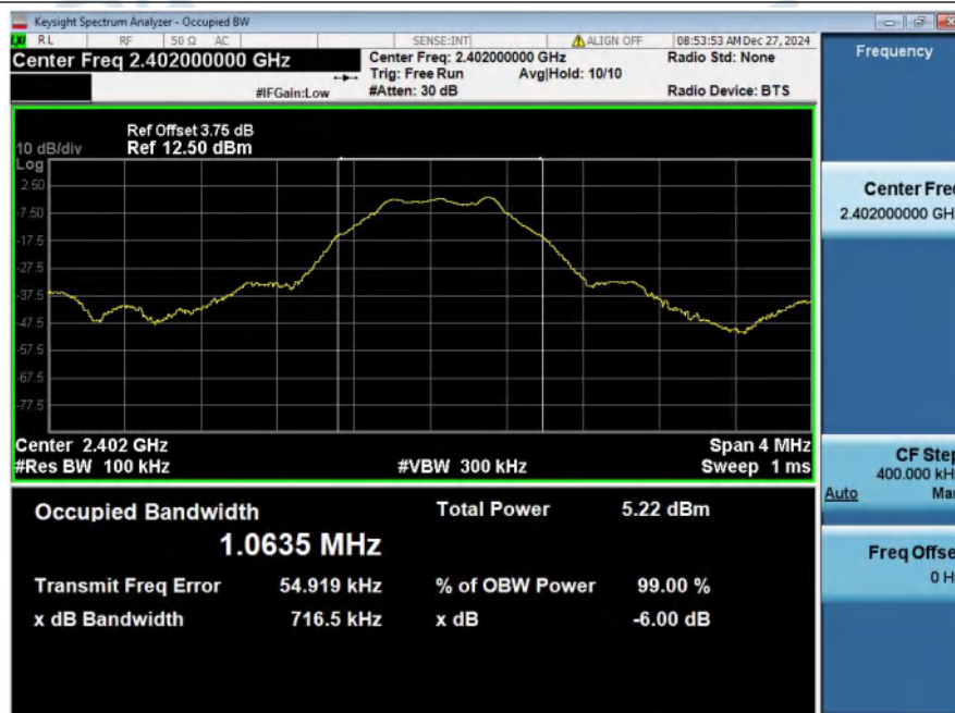
-6dB_Bandwidth_NVNT_ANT1_1Mbps_2402
