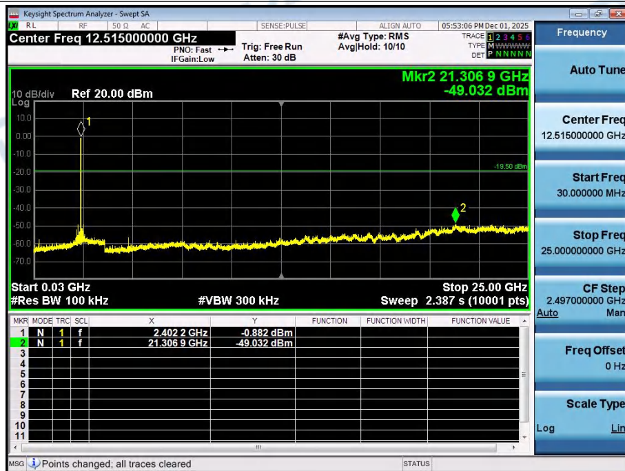
2_Spurious_Emission_BLE_1Mbps_2402
