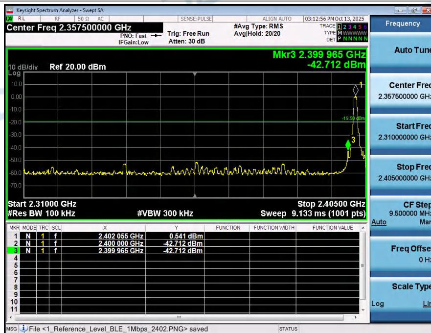
2_Bandedge_BLE_1Mbps_2402
