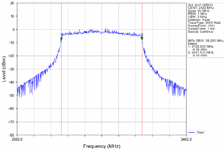
802.11ax(HEW40)_LCH_2422MHz_SU_/_Ant1 (SISO)_NTNV
