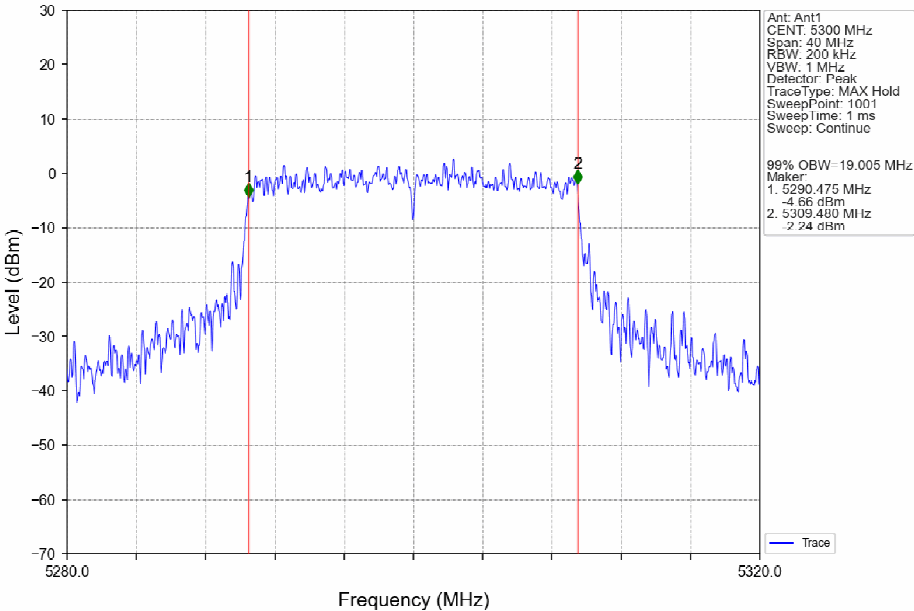
802.11ax(HEW20)_MCH_5300MHz_SU_/_Ant1_NTNV
