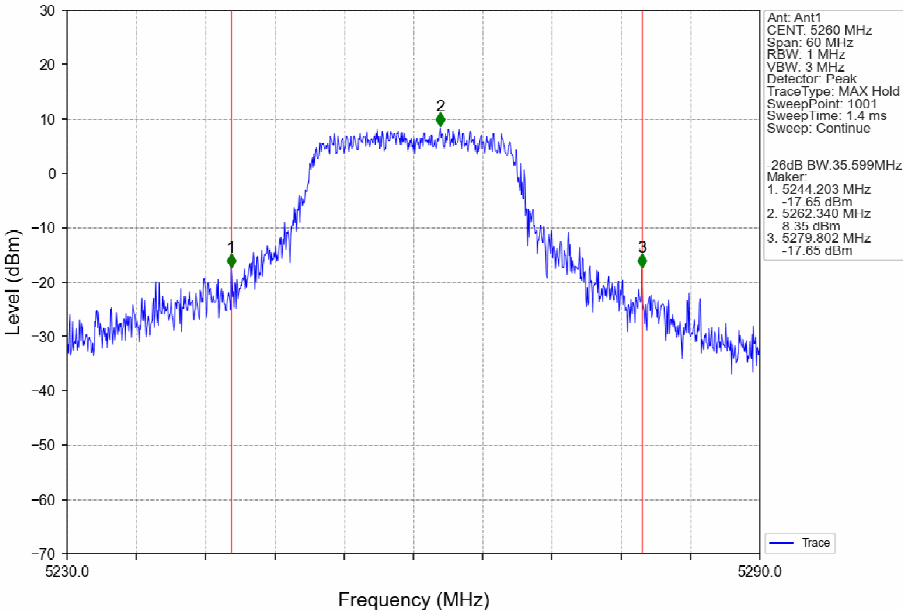
802.11ac(VHT20)_LCH_5260MHz_Ant1_NTNV
