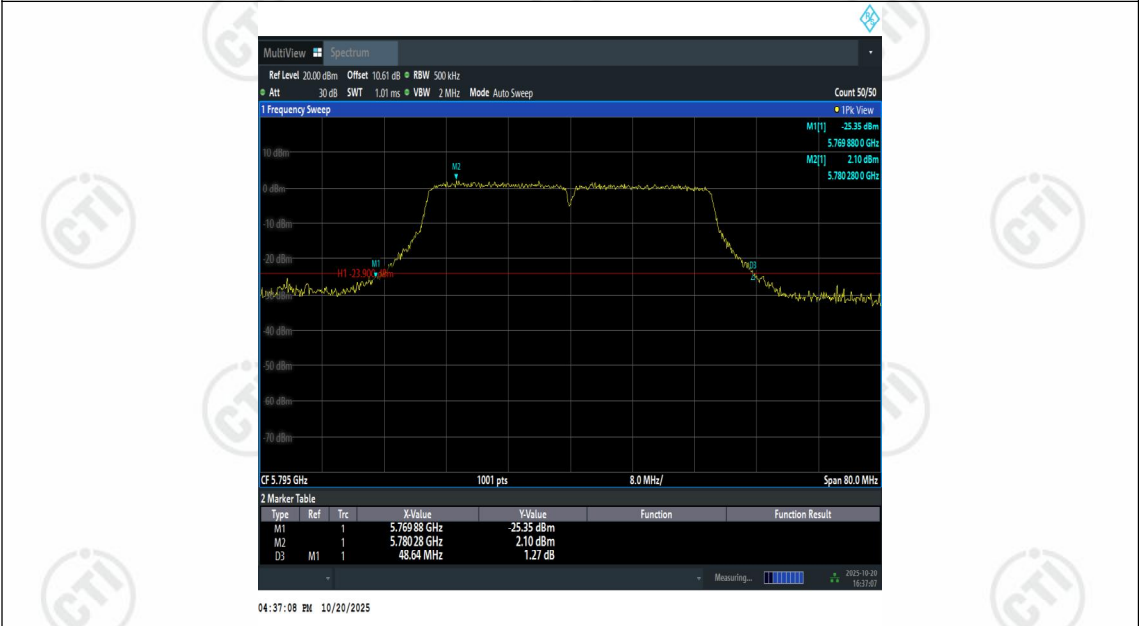
11N40SISO-Ant1-5795
