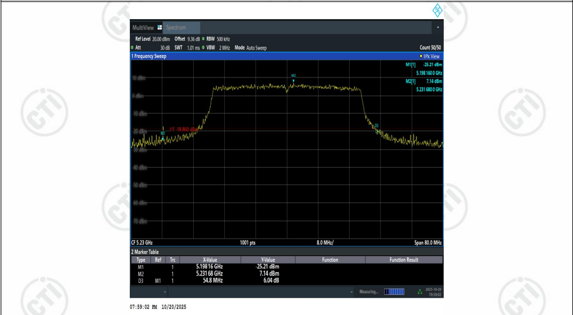
11AX40SISO-Ant1-5230
