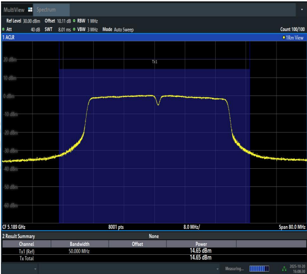
11N40SISO-Ant1-5190-PASS
