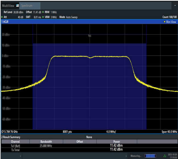
11AC20SISO-Ant1-5785-PASS
