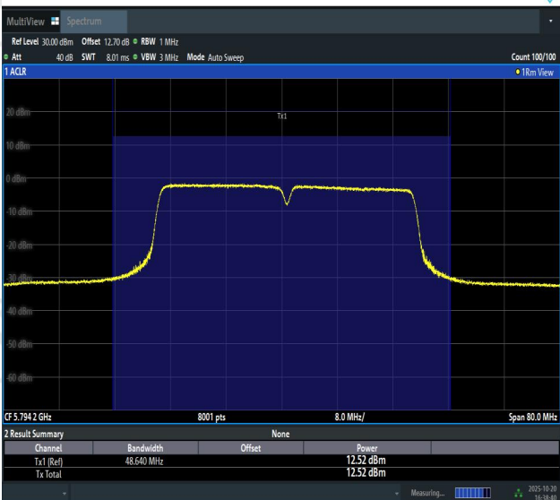
11N40SISO-Ant1-5795-PASS
