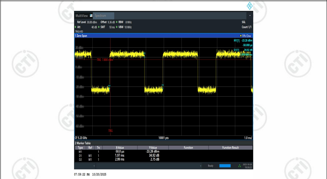
NTNV-11AX40SISO-Ant1-5230
