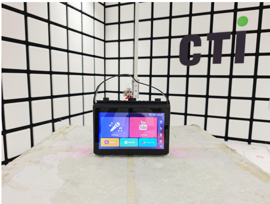
Radiated spurious emission Test Setup-2(1GHz to 18GHz)
