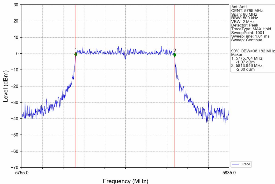
802.11ax(HEW40)_HCH_5795MHz_SU_ / _Ant1_NTNV
