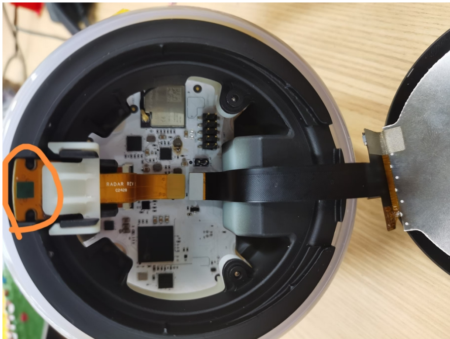
60GHz Radar ANT
