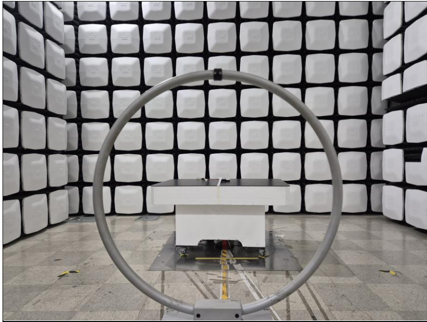
Photo of Radiated Spurious Emission Test (30 MHz ~ 1 GHz)
