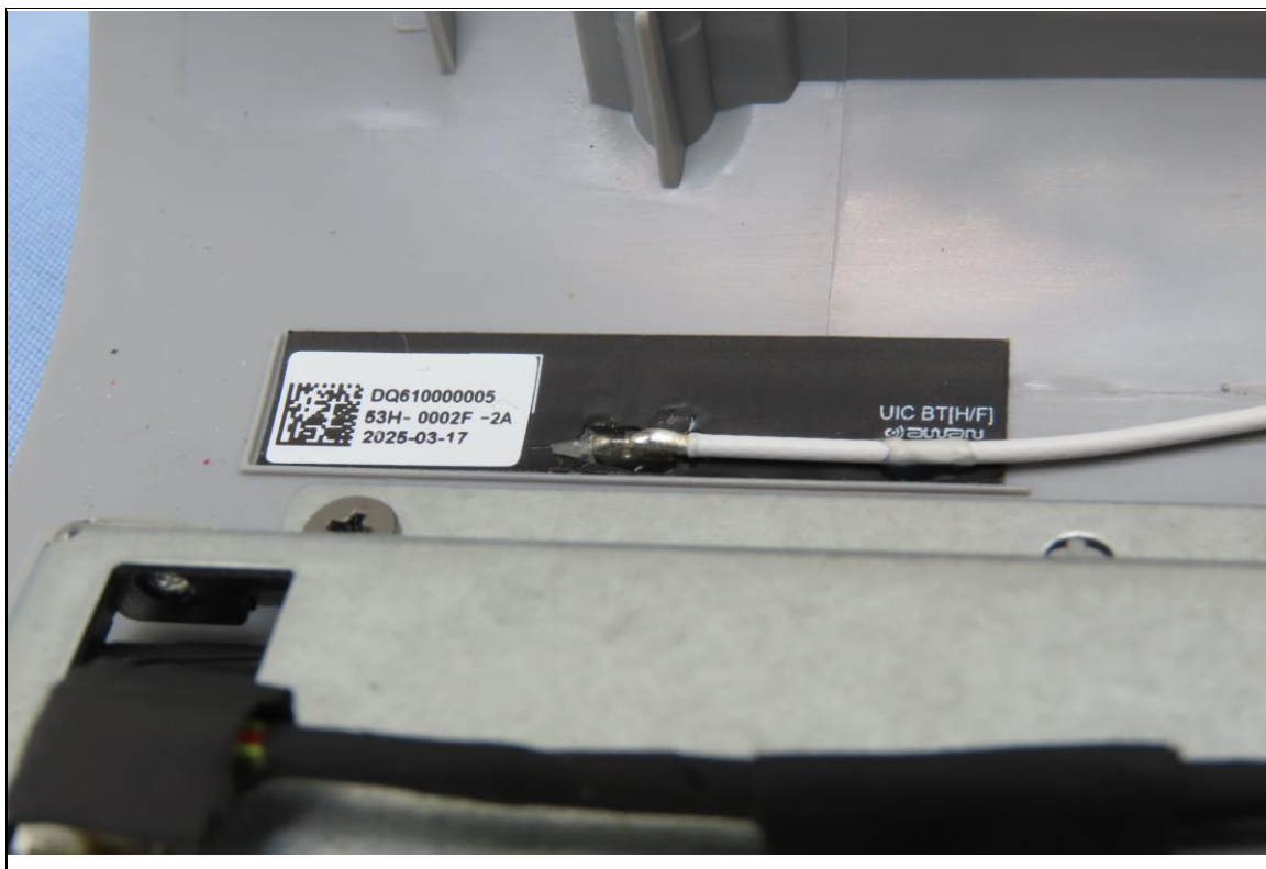
BT Antenna (Brand: Advanced Wireless & Antenna INC. / Model: ABF8P-100000A)
