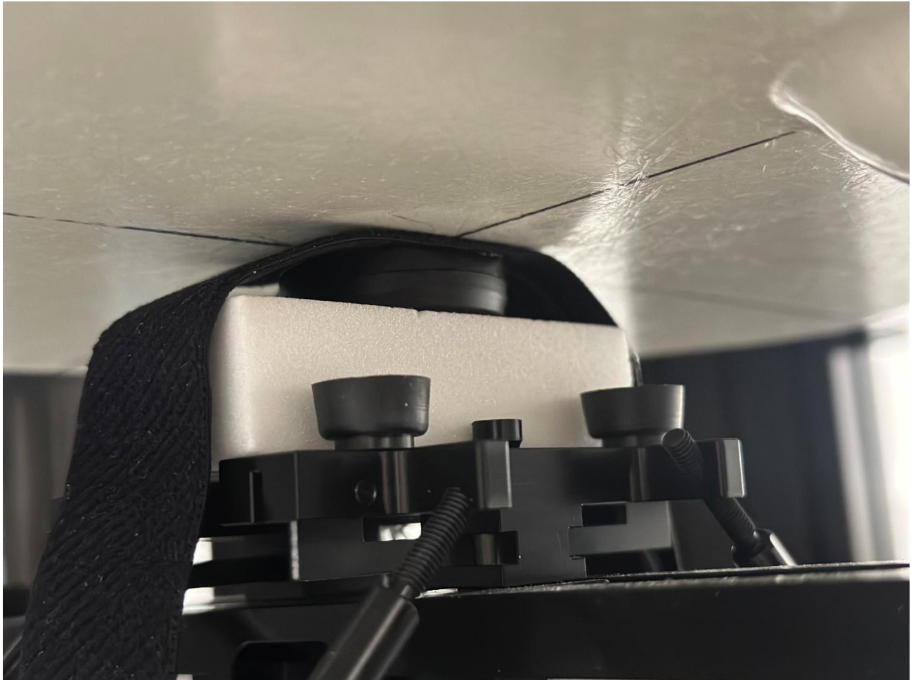
Figure A SAR Test Setup – Body – Back 0mm
