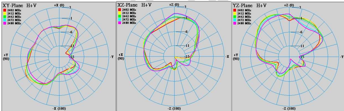
WIFI 2_2402MHz~2480MHz
