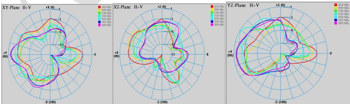
WIFI 2_4910MHz~5850MHz
