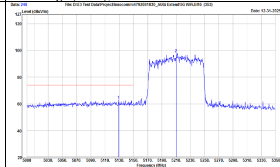
TX, 802.11ac(VHT80) (Ch 42) Band Edge (Peak), Vertical
