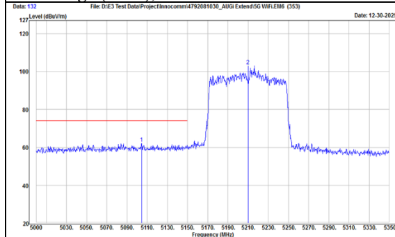
TX, 802.11ac(VHT80) (Ch 42) Band Edge (Peak), Horizontal
