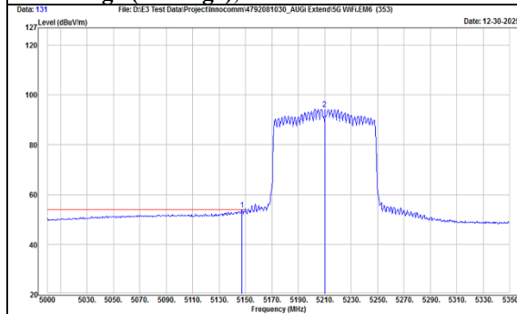
TX, 802.11ac(VHT80) (Ch 42) Band Edge (Peak), Horizontal
