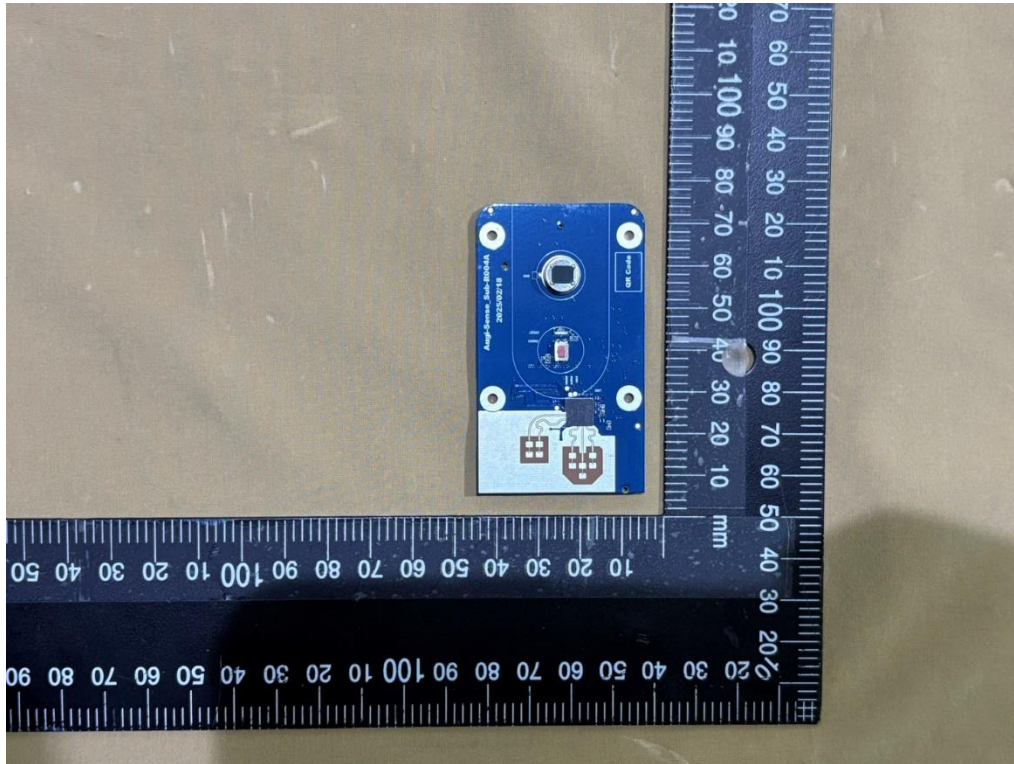
IN6S002 Pic 13
