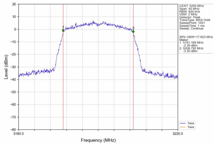
802.11ac(VHT20)_MCH_5200MHz_Ant2_NTNV
