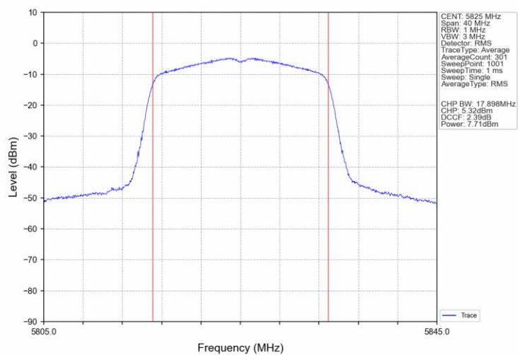
802.11ac(VHT20)_HCH_5825MHz_Ant2_NTNV
