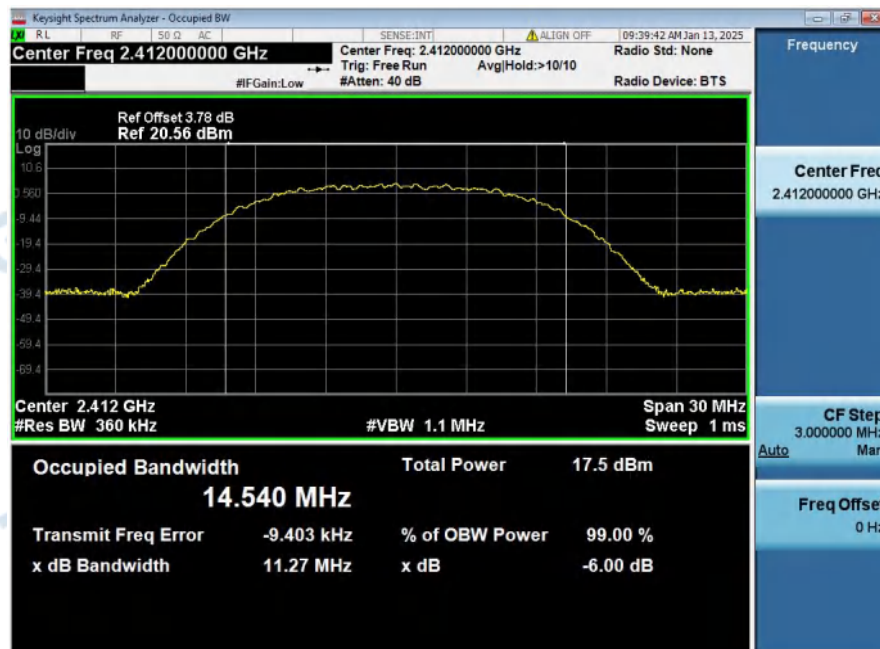
-6dB_Bandwidth_NVNT_ANT1_802_11b_2412
