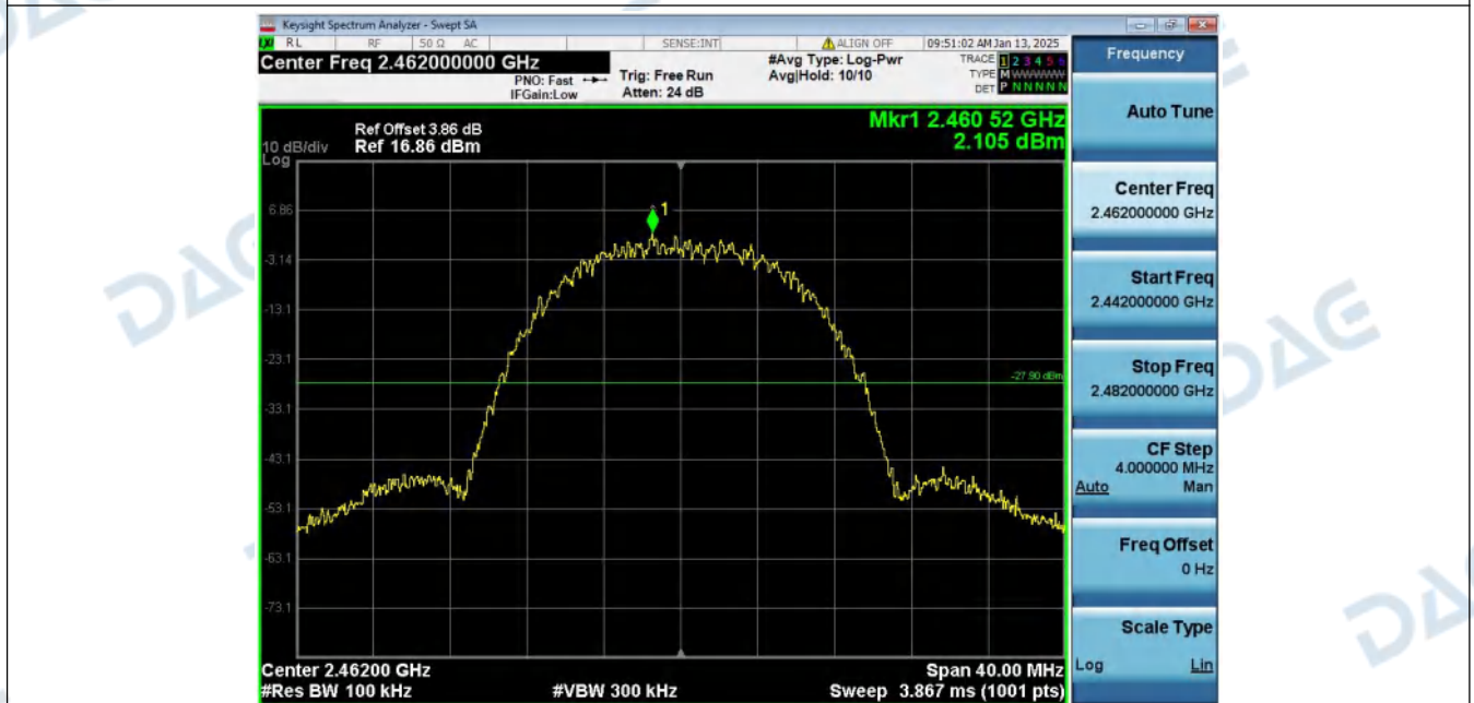
2_Bandedge_NVNT_ANT1_802_11b_2462
