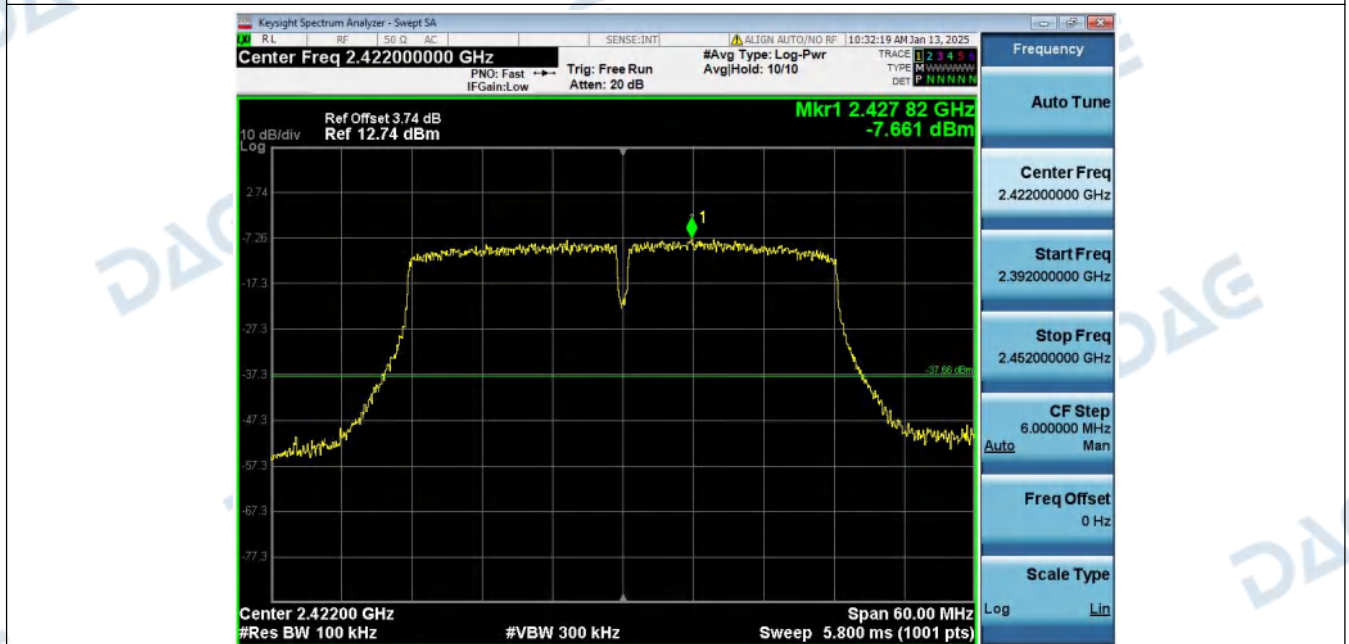
2_Bandedge_NVNT_ANT1_802_11n(HT40)_2422
